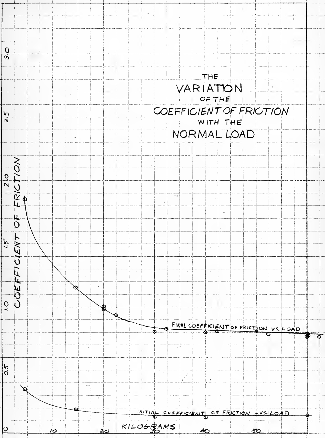
Fig. 6. The coefficient of friction vs. normal load
