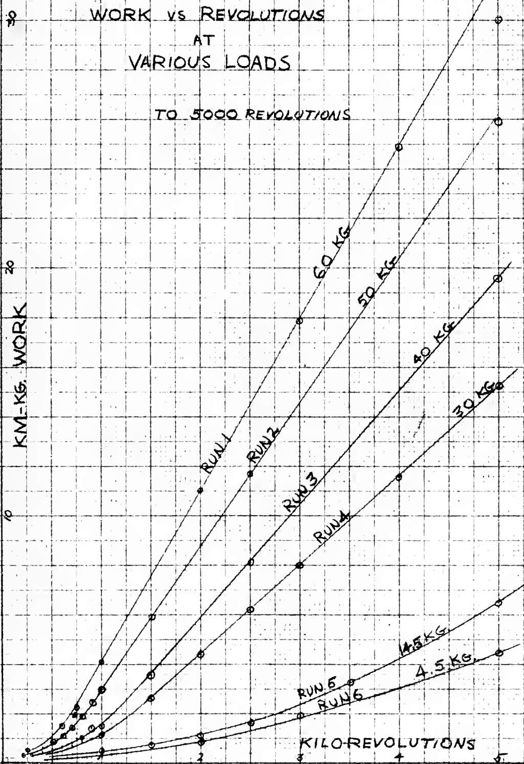
Fig. 4. Work vs. revolutions to 5,000 revolutions
