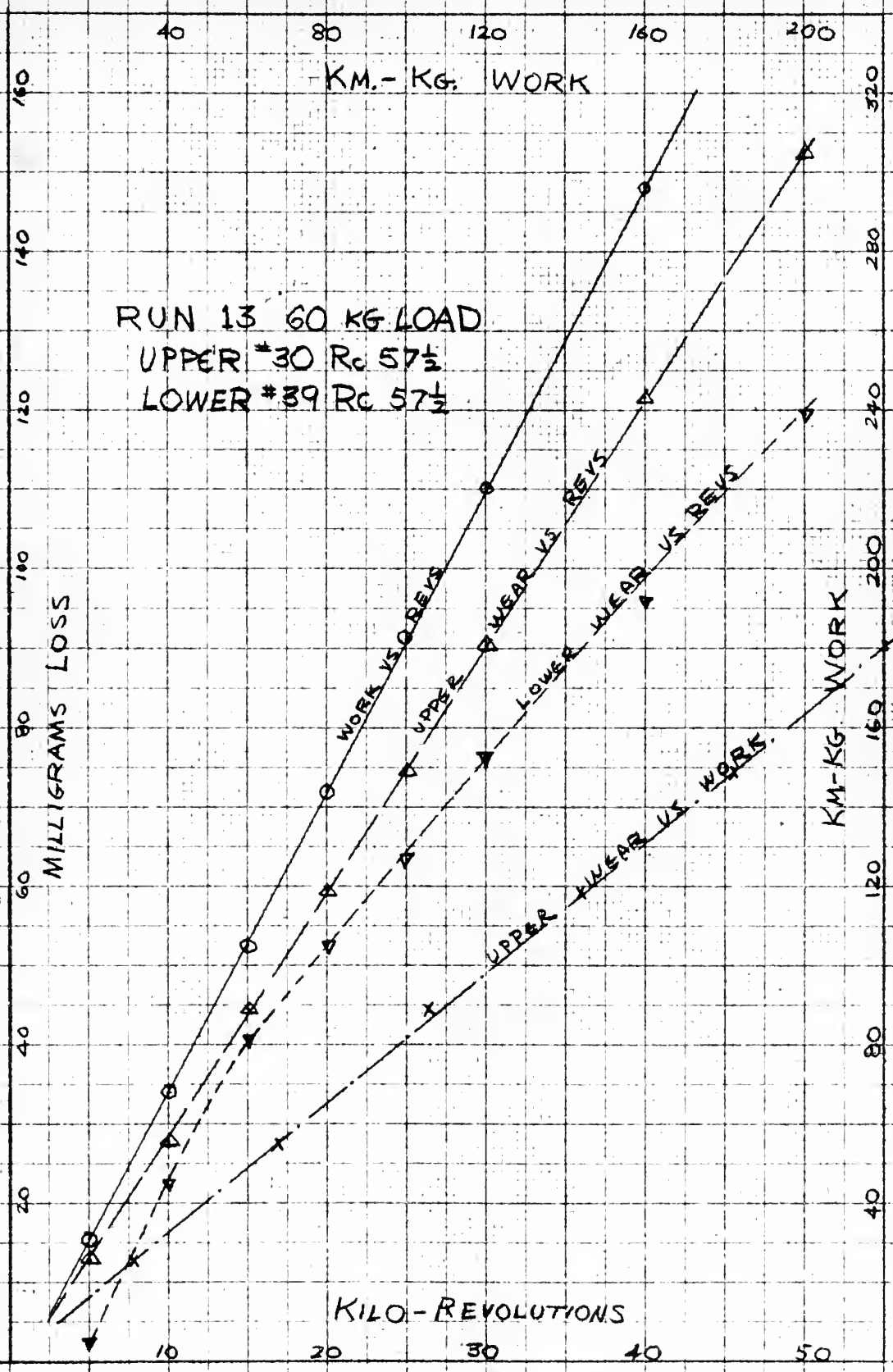
Fig. 28. Curves of results for Run 13 at 60 kg. load
