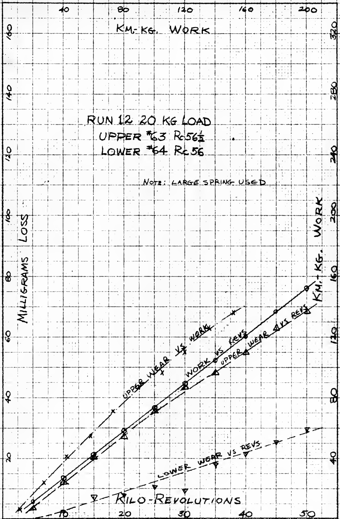
Fig. 27 Curves of results for Run 12 at 20 kg. load
