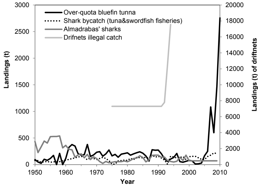
Figure 10. Illegal catch or non-reported catch of vulnerable species (t) (Sources: Raymarkers and Lynham 1999; Silvani et al. 1999; ATRT 2006, 2010; Mielgo Bregazzi 2011).
