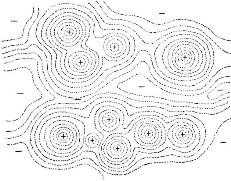
Fig. 1 Dobzhansky's symbolic landscape picture of the relations between the organism and the environment. The picture is a topographic map of all the possible genetic combinations, in which the "contours" follow combinations with equal adaptive values. Adaptive peaks and valleys are marked, respectively, by plus and minus signs [Source Dobzhansky (1937), 3rd ed. 1951, p. 8]
