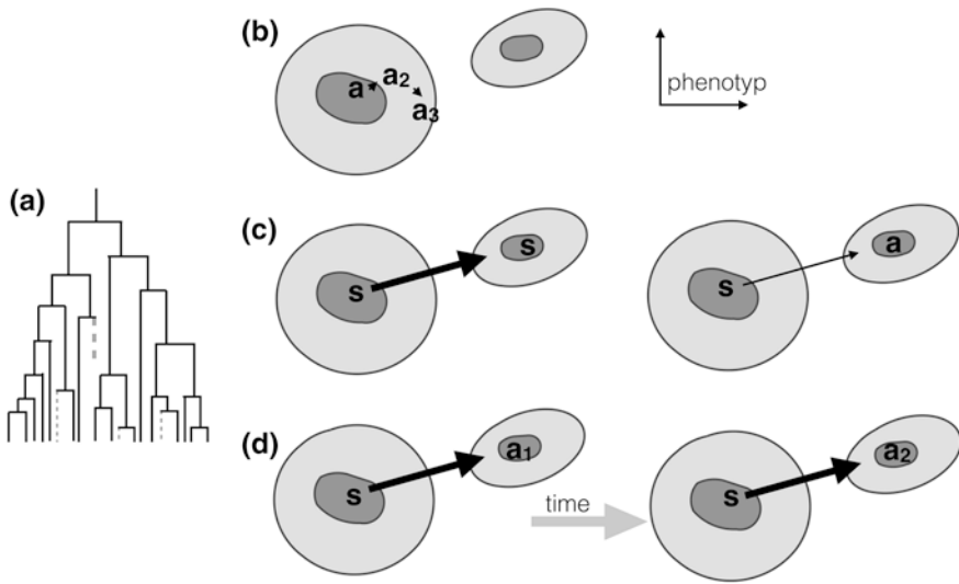
Fig. 3 Schematic of the twig-like distribution and young age of asexual lineages ( a ) and the suggested (micro)-evolutionary mechanism creating this distribution shown on adaptive landscapes ( b–c ). The potential underlying mechanisms are depicted on an adaptive landscape with fitness as a function of two different phenotypic traits ( right ) in a and the differences in fitness indicated by different shades of gray representing higher fitness. Populations are shown as s (sexual) and a (asexual), and subscripts indicate changes over time. Initially, only one fitness peak is occupied. a Asexual lineages (gray dashed lines) evolved independently several times from sexual ancestors (black lines) and got eventually extinct (wide gray dashed line). b The traditional view is that the young age of asexuals results from clonal decay and thus high extinction rates. Over time, the accumulation of deleterious mutations moves the population from a fitness peak till the population goes extinct. Alternative hypothesis explain the young age and twig-like distribution of asexuals with c low transition rates from sexual to asexual reproduction: The open fitness peak is more likely to be occupied by a sexual species ( s , wide arrow) than by an asexual species ( a , narrow arrow). d A high lineage turnover of asexuals results in young ages of asexuals, because new asexual lineages ( a 2 ) are recurrently created from related sexuals and the new lineages replace already existing asexual lineages ( a 1 ) that got extinct by chance
