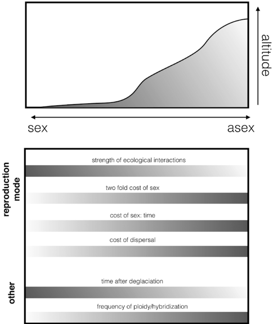
Fig. 4 Schematic of the geographic parthenogenesis ( top panel ) and (micro)-evolutionary processes ( bottom panel ) that have been suggested explaining the distribution of asexuals, which tend to inhabit extreme habitats, e.g., high altitudes and sexuals, which are often missing in the extreme habitats. Traditional explanations link the geographic distribution to benefits and costs of sex: sex can provide an advantage when coevolving with other species, e.g., parasites and because species interactions are less/weaker in extreme habitats, the costs of sex are not balanced under these conditions. Because the costs of sex are more easily balanced in stable habitats (here low altitudes ), sexuals are less often found in the unstable high altitude habitats. Other explanations (reproduction mode independent) are based on higher levels of polyploidy and hybridization and the time after deglaciation (see text)
