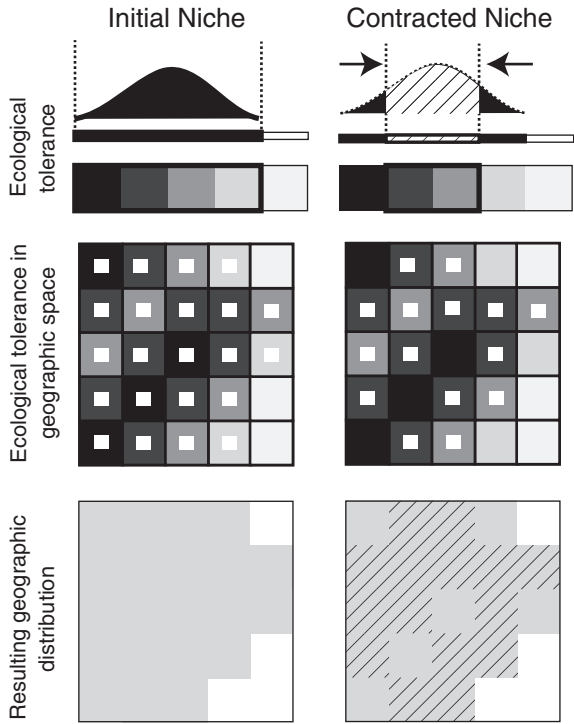
Fig. 10 Relationship between niche evolution in environmental parameter and geographic space. The left column displays the initial environmental tolerance of a species along environmental gradient ( dark to light gray ) and the resulting geographic distribution. The column on the right indicates how contraction of the initial niche can result in high niche similarity but low geographic similarity. Modified from Brame and Stigall (2014)
