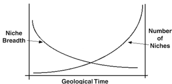
Fig. 1 General view of Hutchinsonian ecological niches through geological time, based on developmental logic
