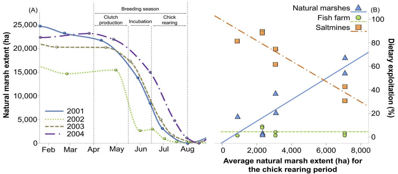
Figure 3. Linking natural resource availability with fledglings' diet. (A) Temporal trends for the flooded areas (ha) at the natural marshes for the 2001–2004 period. Dots represent real flooded areas obtained from satellite images. (B) Relationship between the estimated flooded area at the natural marshes (ha) during the chick-rearing period and the estimated relative contribution of natural resources (blue), and resources from the fish farm (green) and the saltmines (orange) to the diet of Slender-billed Gull fledglings. Dots represent dietary estimates for fledglings hatched at different sites and in different years. doi:10.1371/journal.pone.0047551.g003
