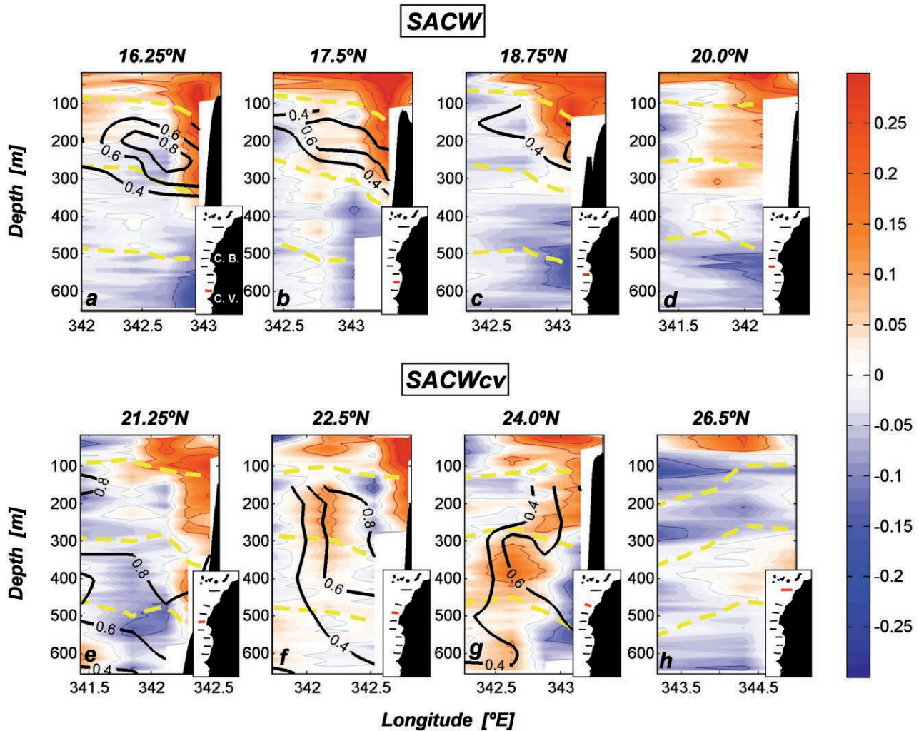
FIG. 4. – Distribution of water masses on eight different cross-shore sections (Fig. 1). The meridional velocity (in [m\ s^{-1}] ) is colour-coded according to the right-hand-side colour bar, with positive values denoting northward flow; contours are drawn every 0.1\ m\ s^{-1} interval. The black lines show either the fraction of SACW south of Cape Blanc (top panels) or the fraction of SACWcv north of Cape Blanc (bottom panels); in the upper panels the remaining water-mass contribution is only SACWcv, while in the lower panels it is NACW. Three selected isopycnals (26.46, 26.85 and 27.1) are drawn in yellow. The map insets indicate the location of the corresponding section.
