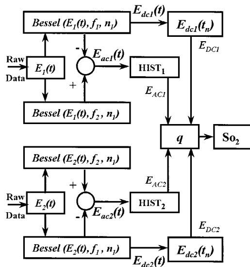
Fig. 5 Flow diagram of the signal processing algorithm showing the operations performed on both channel signals E_1(t) and E_2(t) , Bessel-type low-pass filters [Bessel( E(t), f, n )], histogram reduction filtering (HIST), and the variable E_{AC} and constant E_{DC} values for each wavelength required for the determination of q and SO_2 .
