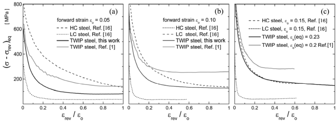
Fig. 4 Evolution of the transient softening for different levels of forward pre-strain. Data extracted from Refs. [1, 12] are included.
