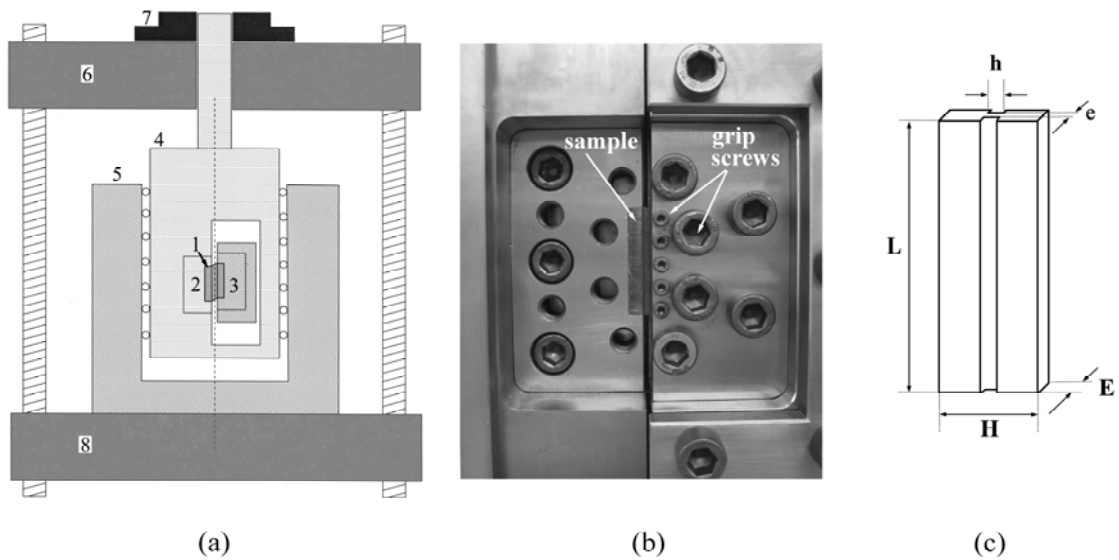
Fig. 2 (a) Schematic overview of the shear test device: 1. sample; 2. movable grip; 3. fixed grip; 4. upper movable frame part; 5. lower fixed frame part; 6. test machine crosshead; 7. load cell; 8. test machine floor. (b) Photograph of the shear device and the grip system. (c) Geometry of shear samples.
