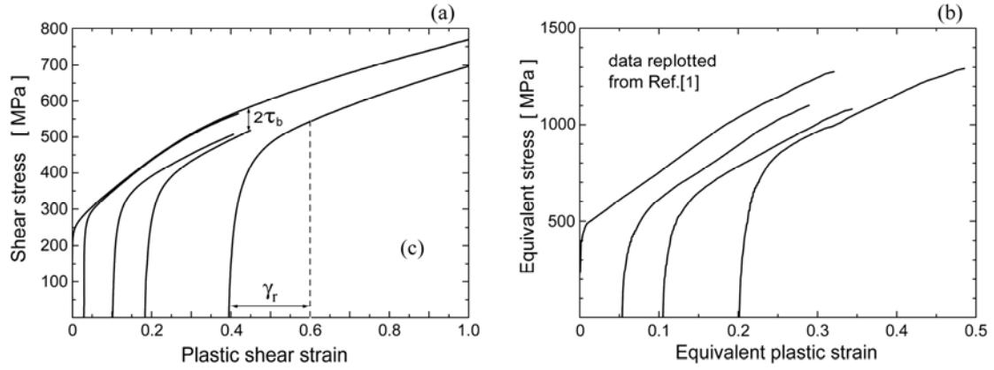
Fig. 3 (a) Bauschinger curves obtained from shear test. Reverse curves are plotted with the flow stress positive to show the permanent softening effect. (b) Data extracted from Ref. [1] and replotted to show the permanent softening effect.
