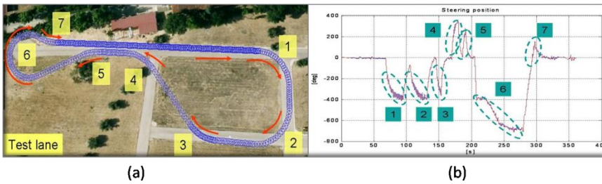
Figure 3. (a) Test lane for buses over the road at IAI-CSIC; (b) Steering wheel position (angle) during an experiment performed on the test lane.
