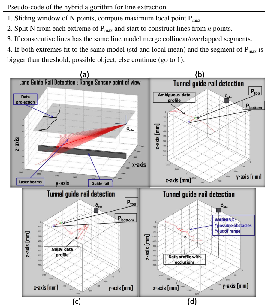
Figure 5. (a) Local laser_rail world frame and its variables; (b) Ambiguous profile; (c) Noisy profile and (d) Data occlusion profile.
