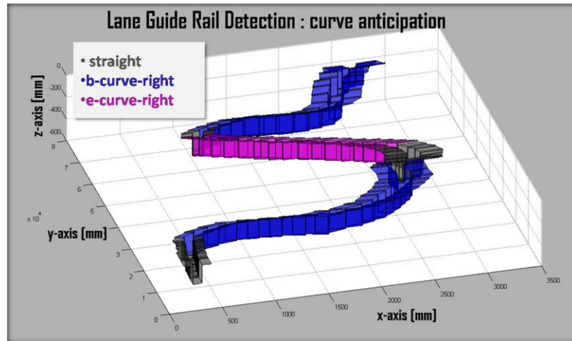
Figure 7. Experimental results of curves anticipation, a 3D representation.
