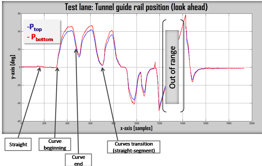
Figure 6. Tunnel guide rail detection, angles at P_{\text{top}} and P_{\text{bottom}} over the entire trajectory (see Figure 3(a)).
