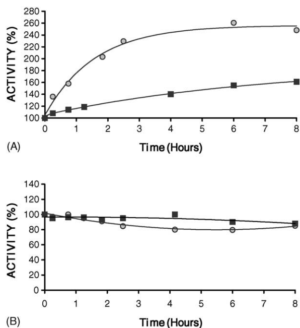
Fig. 1. Variation of the activity of C. rugosa isoenzymes ( 1.3 \times 10^{-5} M) in presence of PEG. Conditions: 4% PEG (w/v) in sodium phosphate buffer (pH 7), 25 °C. (A): ○, lip 3 + PEG 8000; ■, lip 3 + PEG 20,000 and (B): ○, lip 1 + PEG 8000; ■, lip 1 + PEG 20,000.
