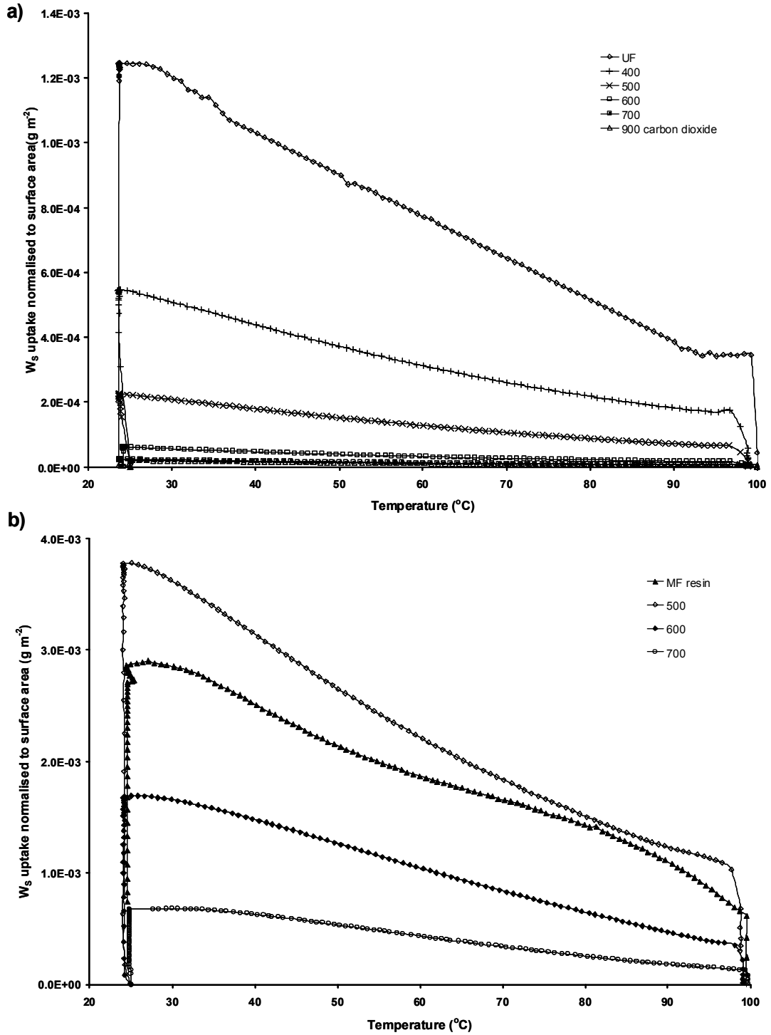
Figure 3. Profiles for \text{CO}_2 uptake normalised by surface area during temperature-programmed \text{CO}_2 adsorption/desorption for a) UF and b) MF derived adsorbents.
