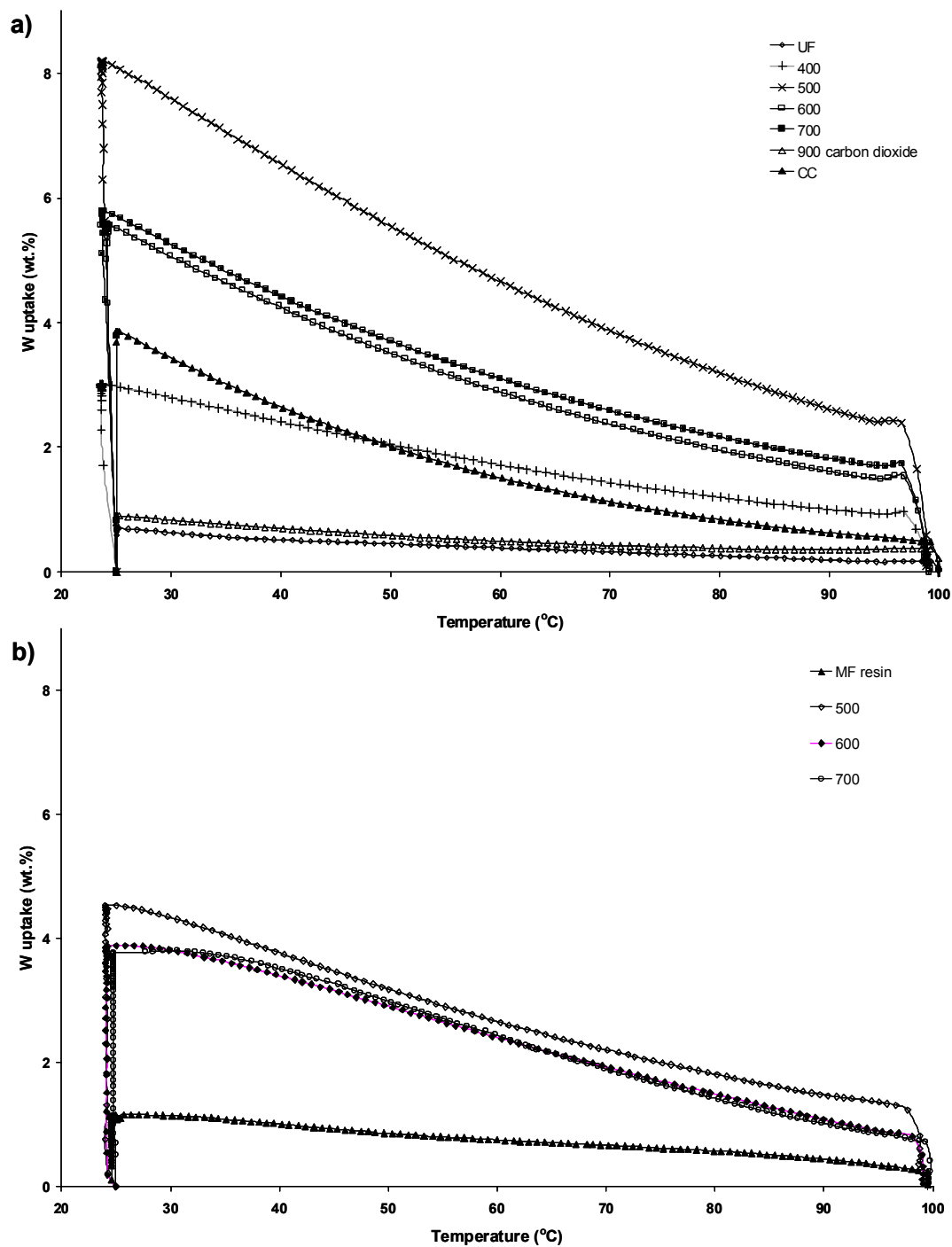
Figure 1. Temperature-programmed adsorption/desorption profiles obtained by CO 2 saturation at room temperature followed by a heating (0.25 °C min -1 from 25 to 100 °C) under CO 2 , and finally, desorption in N 2 at 100 °C for a) UF and b) MF derived adsorbents.
