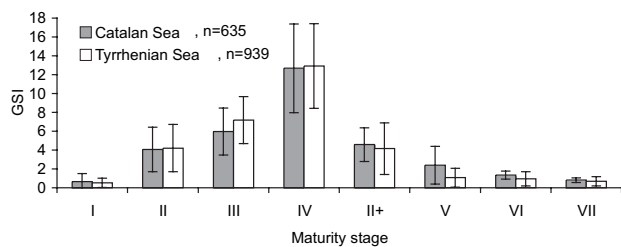
FIG. 5. – Merluccius merluccius mean female gonadosomatic index (GSI) for each maturity stage. Bars denote SD.
