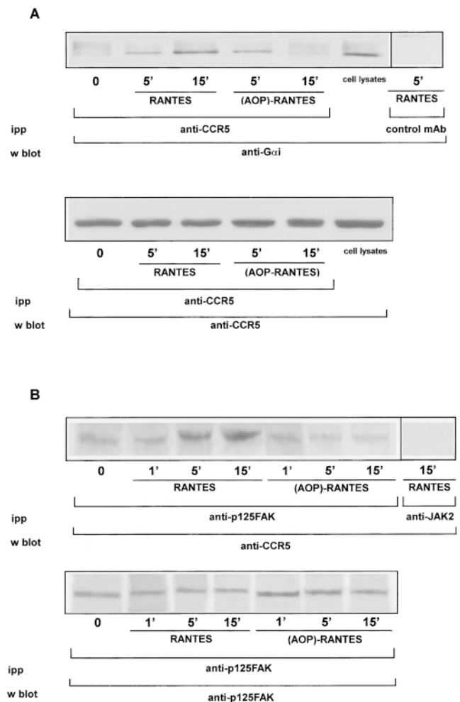
Figure 7. RANTES and (AOP)-RANTES promote G \alpha_i and p 125 FAK association to the CCR5 receptor. (A) 10 nM RANTES or (AOP)-RANTES-induced CCR5-transfected HEK-293 cell lysates were immunoprecipitated with anti-CCR5 (CCR5-03) or with an anti- \beta_2 -microglobulin control mAb, and the Western blot developed with anti-G \alpha_i antibody. As a control for CCR5 loading equivalence, the blot was stripped and reprobed with the anti-CCR5 mAb CCR5-02. As a positive control, CCR5-transfected HEK-293 cell lysates were tested in Western blot with the same anti-G \alpha_i or anti-CCR5 antibodies. (B) CCR5-transfected HEK-293 cells were stimulated with RANTES or (AOP)-RANTES as in A. Cell lysates were immunoprecipitated with anti-p 125 FAK, or anti-JAK2 antibodies as control, the Western blot developed with anti-CCR5 mAb CCR5-02. Protein loading was controlled by stripping the membrane and reprobing with anti-p 125 FAK antibody.
