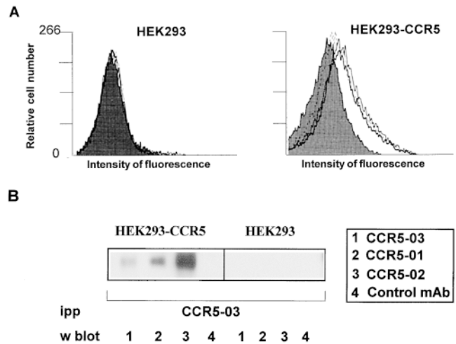
Figure 1. CCR5-01, -02, and -03 antibodies are specific for the CCR5 chemokine receptor. mAb specificity for the CCR5 receptor was assessed by flow cytometry analysis of mock- and CCR5-transfected HEK-293 cells. (A) CCR5-transfected HEK-293 cells (HEK-293-CCR5) or mock-transfected controls (HEK-293) were incubated with the biotin-labeled CCR5-01, -02, or -03 antibodies, followed by streptavidin-PE. An isotype-matched mAb was used as a control. (B) CCR5- or mock-transfected HEK-293 cells were immunoprecipitated as described in Materials and Methods using CCR5-03 mAb, then analyzed in Western blot with CCR5-01, -02, -03, or control mAb, as indicated. One representative experiment of five is shown.
