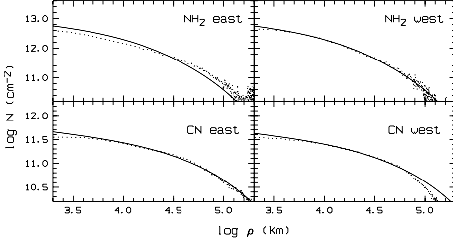
Fig. 4. CN and NH 2 column density profiles of Comet Lee (dots) in the east-west direction. The solid lines represent the results obtained by means of the Haser model with equivalent scalelengths and production rates listed in Table 2 for CN (1–0) and as mentioned in the text for NH 2 .
