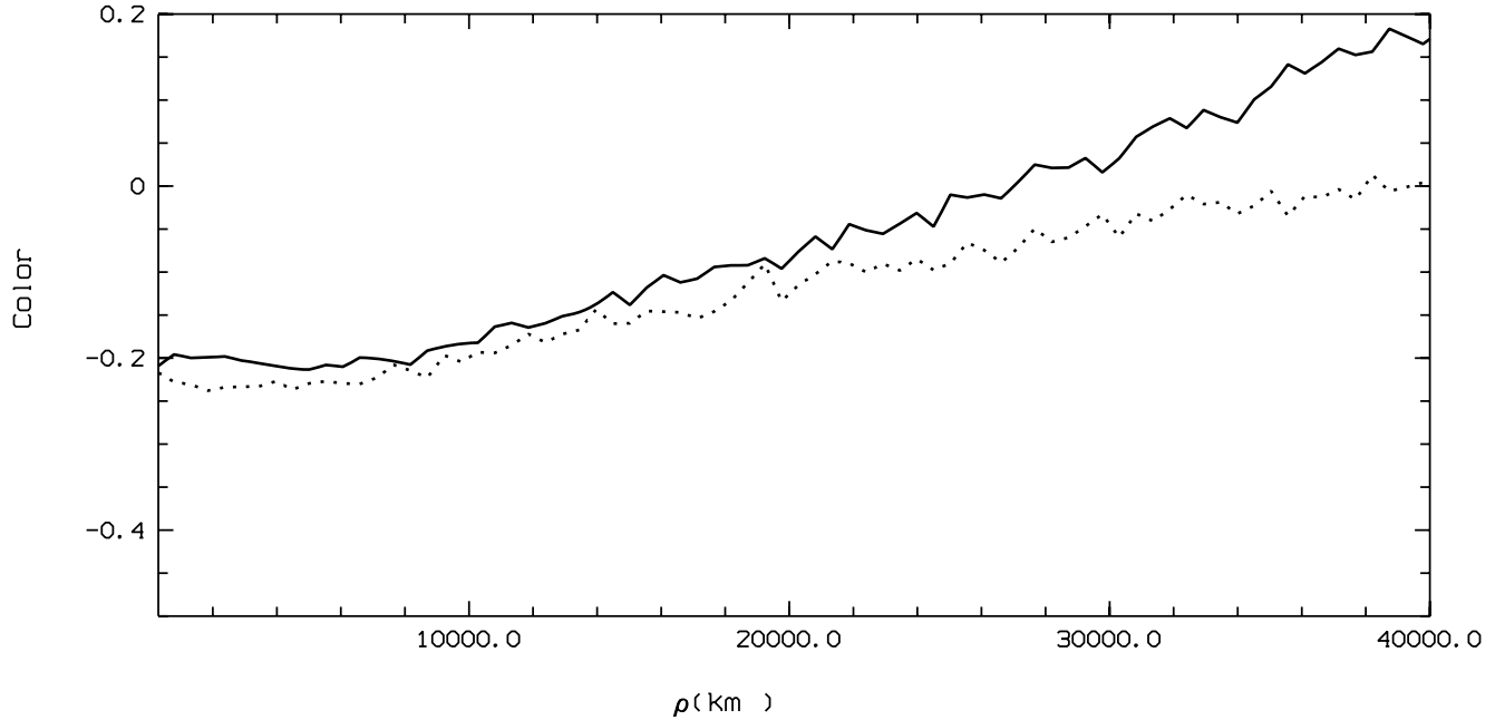
Fig. 6. Color of the dust in the coma of C/1999 H1 (Lee) in the west (solid line) and east (dotted line) direction as computed from Eq. (1) for 8400 \leq \lambda_L \leq 8500 \text{ \AA} and 6800 \leq \lambda_S \leq 6900 \text{ \AA} . Note the increasing reddening of the dust at \rho \geq 10000 \text{ km} in both directions. At larger cometocentric distances, the differences in east-west direction cannot be attributed to significant variations in the physical and/or chemical properties of the cometary dust since at \rho > 30000 \text{ km} the error due to the contribution of the sky is getting larger.
