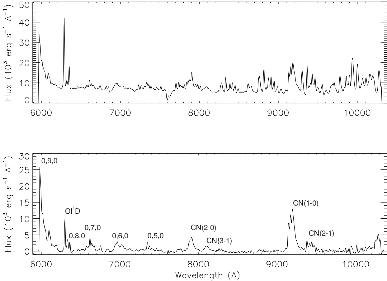
Fig. 3. Observed and gas spectrum of Comet Lee (C/1999 H1) spatially integrated along the slit. In the observed cometary spectrum, the sky values have not been subtracted so that it clearly shows the oxygen telluric line, the O 2 B and A bands at ~6800 and ~7600 Å, H 2 O at ~8200 Å, and OH band longward 9000 Å. In the lower panel, pure cometary emissions is seen: the CN red system as well as the (0, \nu_2 , 0) NH 2 bands (with the blended OI lines at 6300 Å and at 6364 Å).
