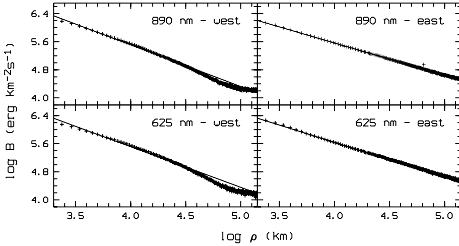
Fig. 5. Brightness profiles of Comet Lee in two different continuum regions. The profiles were obtained from the median averaged spectrum in the east-west direction, representing approximately the sun-tail direction. The surface brightness, B , is plotted against the projected radius, \rho in double logarithmic representation. Dots represent the observed profiles and the solid lines are the best fits verifying \frac{d(\log B)}{d(\log \rho)} = -m starting at \log \rho \geq 3.2 , with slopes listed in Table 3.
