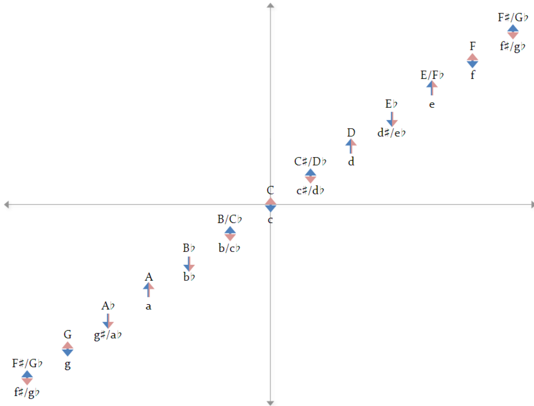
Figure 2: Tonal activities (due to parallel comparisons) of all possible triad pairings.
