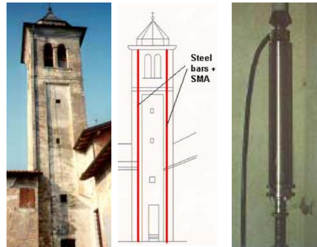
Figure 18. Bell Tower of S. Giorgio Church in Trignano; retrofit intervention with vertical SMA wires in series with prestressed steel tendons and detail of the device (Indirli 2000)
