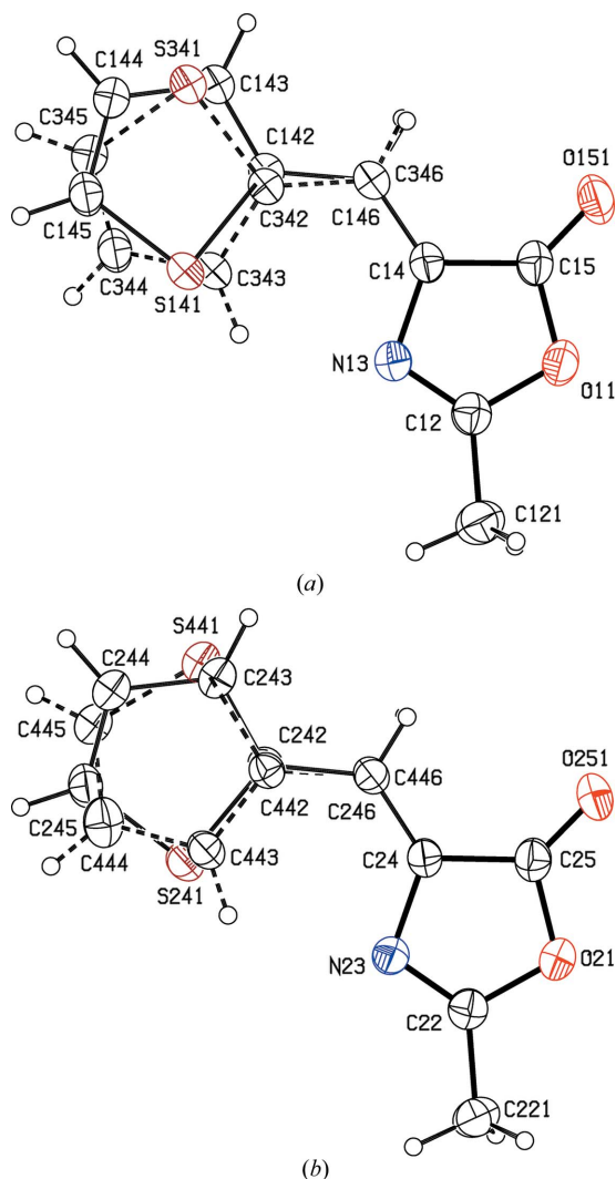
Figure 2 The molecular structures of the two independent and disordered molecules in compound (II), showing the atom-labelling schemes, for (a) a type 1 molecule where the site occupancies of the disorder components are 0.974 (2) and 0.026 (2), and (b) a type 2 molecule where the site occupancies of the disorder components are 0.931 (2) and 0.069 (2). The atomic coordinates of sites C146 and C346 are identical, as are those of sites C246 and C446, although those of the associated H atoms are not identical. Displacement ellipsoids are drawn at the 30% probability level.
