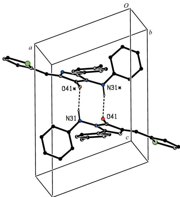
Figure 9 Part of the crystal structure of compound (IV), showing the formation of a hydrogen-bonded R_2^2(10) dimer centred at (\frac{1}{2}, \frac{1}{2}, \frac{1}{2}) . For the sake of clarity, the minor disorder components and H atoms not involved in the motif shown have been omitted. Atoms marked with an asterisk (*) are at the symmetry position (-x + 1, -y + 1, -z + 1) . Note the different orientations of the unit-cell outlines in Figs. 8 and 9.
