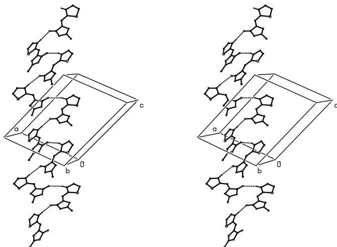
Figure 7 A stereoview of part of the crystal structure of compound (II), showing the formation of a hydrogen-bonded C_2^2(14) chain running parallel to [101] . For the sake of clarity, the minor-disorder components and H atoms not involved in the motif shown have been omitted.
