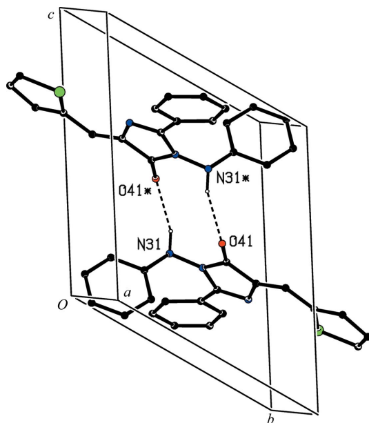
Figure 8 Part of the crystal structure of compound (III), showing the formation of a hydrogen-bonded R_2^2(10) dimer centred at (\frac{1}{2}, \frac{1}{2}, \frac{1}{2}) . For the sake of clarity, the minor disorder components and H atoms not involved in the motif shown have been omitted. Atoms marked with an asterisk (*) are at the symmetry position (-x + 1, -y + 1, -z + 1) . Note the different orientations of the unit-cell outlines in Figs. 8 and 9.
