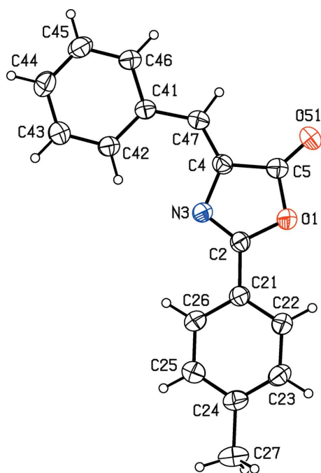
Figure 1 The molecular structure of compound (I) in the triclinic polymorph, showing the atom-labelling scheme. Displacement ellipsoids are drawn at the 30% probability level.
