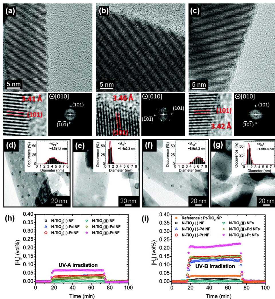
Figure 5. HR-TEM images of (a) pristine and (b, c) N-doped \text{TiO}_2 nanofibers obtained after annealing acid washed sodium titanate nanofibers in \text{NH}_3 . Images (d)–(g) display TEM micrographs of N-doped and then Pd or Pt decorated NFs with metal loading of approx. 1.0 wt%. Panels (h) and (i) show hydrogen evolution from ethanol/water mixture (molar ratio 1:3) over the corresponding photocatalyst materials under UV-A and UV-B irradiation, respectively. Reproduced from [123]. Copyright 2011 American Chemical Society.
