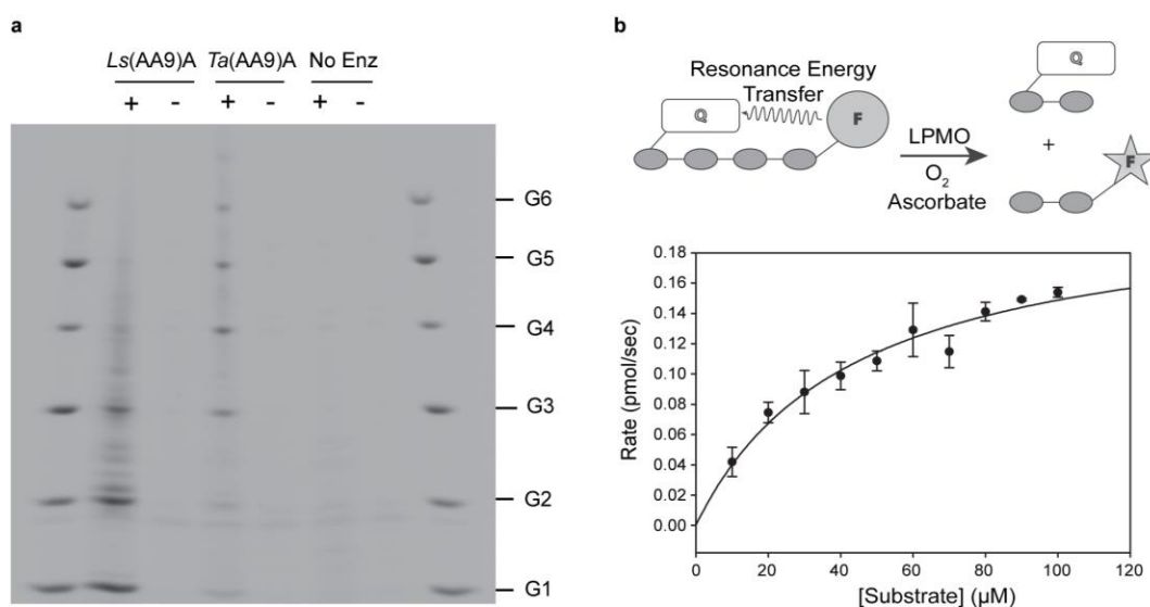
Figure 2 | Ls (AA9)A and Ta (AA9)A activities on insoluble and soluble cellulose. a, Comparison of Ls (AA9)A and Ta (AA9)A activities on PASC. Reaction products were analyzed by PACE (performed in triplicate). +, incubation with ascorbate; –, incubation without ascorbate. b, Cleavage of FRET substrate by Ls (AA9)A and subsequent Michaelis-Menten plot, error bars represent random error of triplicate measurements.
