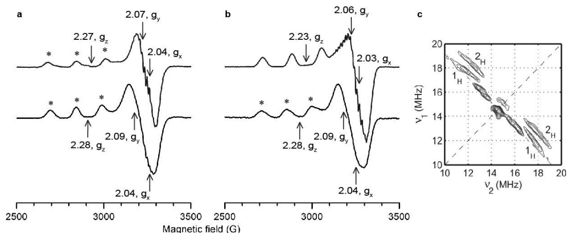
Figure 5 | EPR spectra of Ls(AA9)A . * indicates signals from copper site where water was the exogenous ligand, other signals were from species with chloride as exogenous ligand. a , X-band cw EPR spectra in low chloride conditions, Ls(AA9)A –G6 (top) and Ls(AA9)A with no oligosaccharide (bottom). b , X-band cw EPR spectra in high chloride conditions, Ls(AA9)A –G6 (top) and Ls(AA9)A with no oligosaccharide (bottom). c , Contour presentation of the ^1\text{H} -HYSCORE spectrum of Ls(AA9)A –G6 in the presence of chloride ions (magnetic field 343.6 mT, time between first and second pulse \tau = 136 ns,
