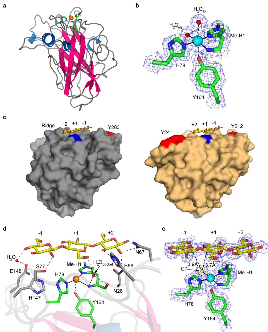
Figure 3 | Structural views of Ls (AA9)A with the copper ion depicted as an orange sphere, Cu(I); or a blue sphere, Cu(II). a , Ribbon view of Ls (AA9)A. b , Electron density of active site obtained with low X-ray dose. c , Comparison of Ls (AA9)A (left) and Ta (AA9)A (right) surfaces. Ls (AA9)A–G3 (lowdose) with Tyr203 in red. Ta (AA9)A
