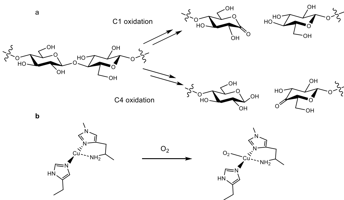
Figure 1 | LPMO activity and active site. a , Oxidative cleavage of a polysaccharide chain carried out by LPMOs, showing different routes of oxidation carried out by different sub-groups of LPMOs. 23 b , The histidine brace active site and proposed first step in the reaction with oxygen. 18
