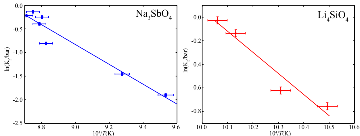
Figure 7: Plot of \ln(K_p) against the inverse decomposition onset temperatures derived from TPD experiments for \text{Na}_3\text{SbO}_4 and \text{Li}_4\text{SiO}_4 . The linear fit to determine the constants A and B relating to K_p is also shown on each plot.
