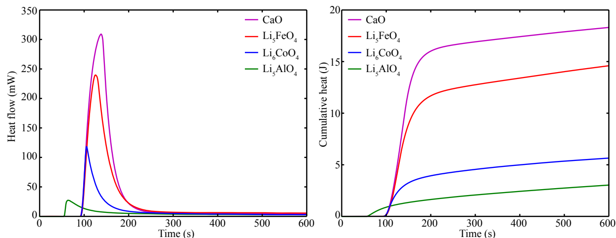
Figure 9: DSC obtained heat flow and cumulative heat traces for CaO, Li 5 FeO 4 , Li 6 CoO 4 and Li 5 AlO 4 samples, studied isothermally at 823 K under p(\text{CO}_2) = 1 bar. There is a lag of \sim 60 - 100 s before carbonation begins due to the change of reactive gas flow in the TGA between pure N 2 and pure CO 2 . The difference in lag between the trace for Li 5 AlO 4 and the other samples is due to the use of a slightly different gas flow setup which uses valves to change between gases more quickly.
