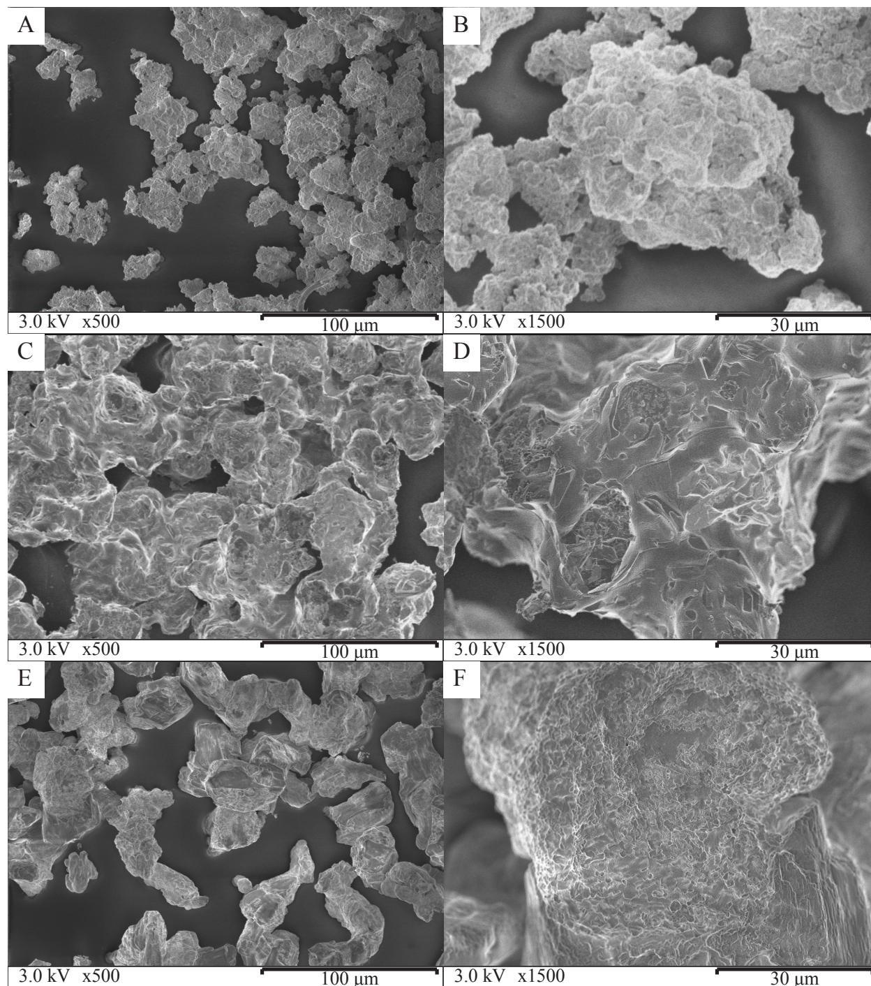
Figure 11: SEM images of \text{Na}_3\text{SbO}_4 samples under two different magnifications (left: x500, right: x1500): heated to 1223 K under \text{N}_2 (a) and (b); fully carbonated (c) and (d); and cycled 20 times, then fully regenerated under \text{N}_2 (e) and (f). Upon extended cycling \text{Na}_3\text{SbO}_4 shows a drastic decrease in both surface area and available porosity, which is likely responsible for its reduction in cycling capacity. The drastic reduction in surface area can be seen especially in the cycled material (f) as compared to the unreacted material (b), indicating that this is a key parameter influencing the cycling stability of \text{Na}_3\text{SbO}_4 .
