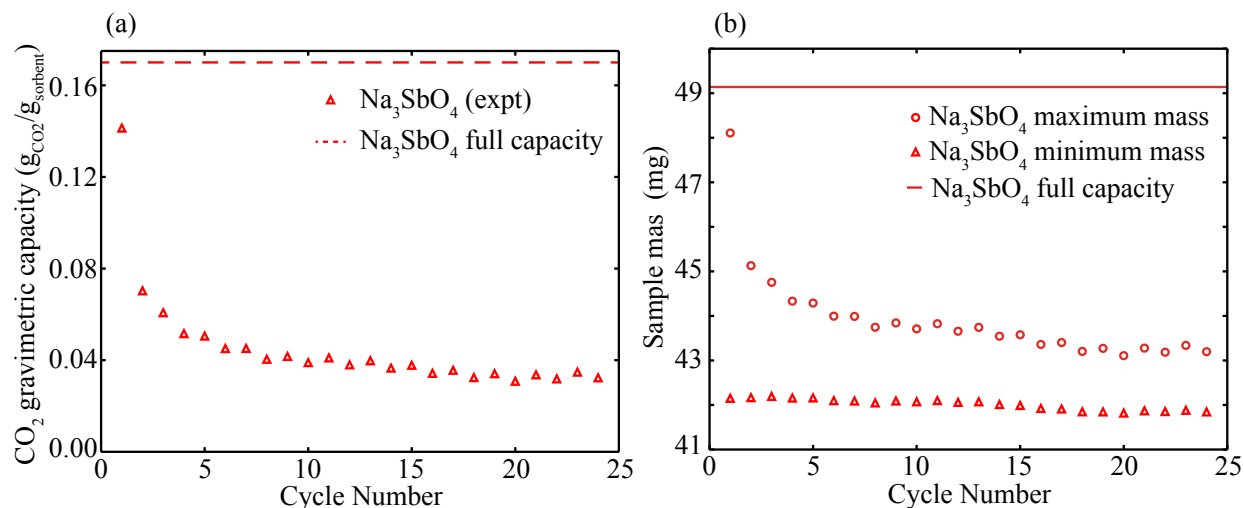
Figure 10: (a) Gravimetric CO 2 capacity as a function of cycle number for Na 3 SbO 4 , measured by TGA under p(\text{CO}_2) = 0.1 bar. The full and dashed lines show the predicted capacity, based on the stoichiometry of the carbonation reaction. Na 3 SbO 4 initially absorbs CO 2 at close to full theoretical capacity, but its capacity quickly fades to between 25–35 % of that of the first cycle. (b) Maximum and minimum sample masses measured during each cycle for Na 3 SbO 4 .
