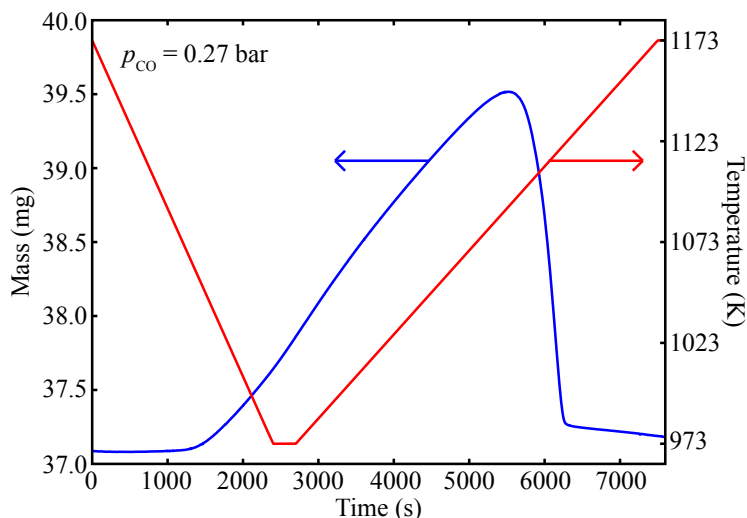
Figure 6: Temperature programmed decomposition (TPD) experiment for \text{Na}_3\text{SbO}_4 at p_{\text{CO}_2} = 0.27 bar. The mass gain corresponds to the carbonation reaction \text{Na}_3\text{SbO}_4 + \text{CO}_2 \rightarrow \text{Na}_2\text{CO}_3 + \text{NaSbO}_3 . Calculation of the zero point of the first derivative of the mass curve gives the temperature of the onset of decomposition.
