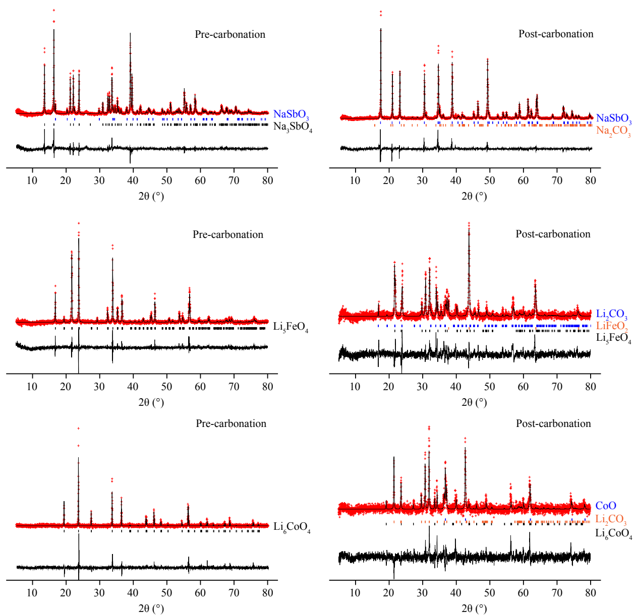
Figure 5: Indexed XRD diffractograms ( \lambda = 1.54056 \text{ \AA} ) and refinements of the as-synthesised \text{Na}_3\text{SbO}_4 , \text{Li}_5\text{FeO}_4 and \text{Li}_6\text{CoO}_4 samples, and after carbonation at 973 K ( \text{Li}_5\text{FeO}_4 and \text{Li}_6\text{CoO}_4 ) or 1223 K ( \text{Na}_3\text{SbO}_4 ) under p_{\text{CO}_2} = 0.37 bar. The experimental data points are shown in red, with the pattern obtained from the Rietveld refinements overlaid in black, and the difference curve below.
