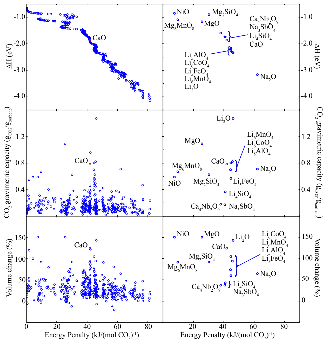
Figure 4: Overview of results from the screening of the Materials Project database for compounds that undergo carbonation. Each data point represents the carbonation reaction for each distinct compound with the most negative \Delta H . The calculated energy penalty, E_p , for each reaction is plotted against \Delta H_{\text{carbonation}} (top), \text{CO}_2 gravimetric capacity (middle) and volume change (bottom). The plots on the left are for the complete 640 distinct compounds in the screening, and the plots on the right are for specific compounds of interest (including the five candidate materials).
