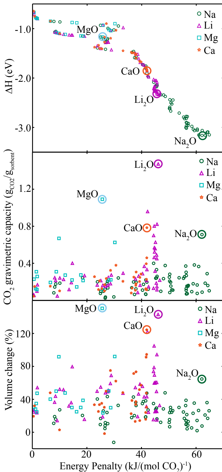
Figure 12: Screened materials containing Na, Li, Mg or Ca as their alkali atom. Each data point represents the carbonation reaction for each distinct compound with the most negative \Delta H . The calculated energy penalty, E_p , for each reaction is plotted against \Delta H_{\text{carbonation}} (top), \text{CO}_2 gravimetric capacity (middle) and volume change (bottom). The respective binary oxides are circled for clarity.
