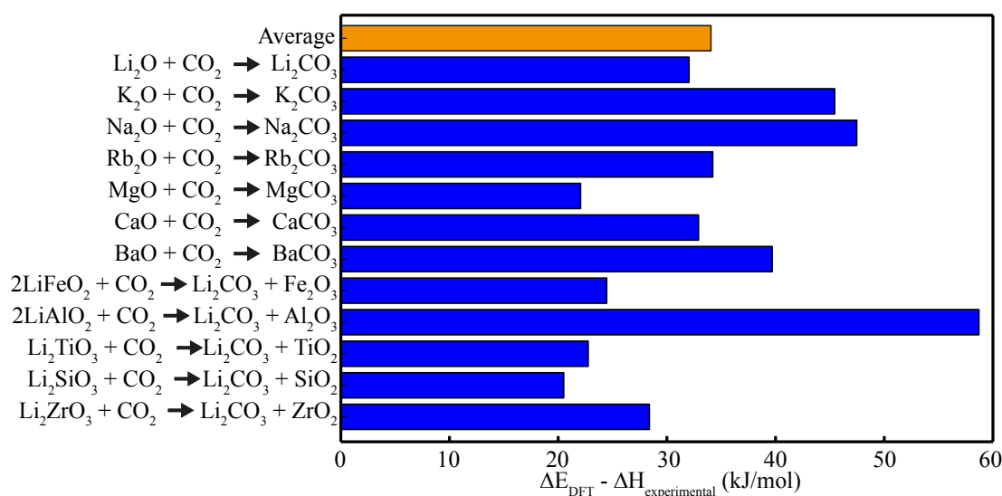
Figure 2: Errors between \Delta E_{DFT} and \Delta H_{experimental} at 293 K for selected binary and ternary oxides. The average error was used as a correction to E_{CO_2} in the Materials Project database.
