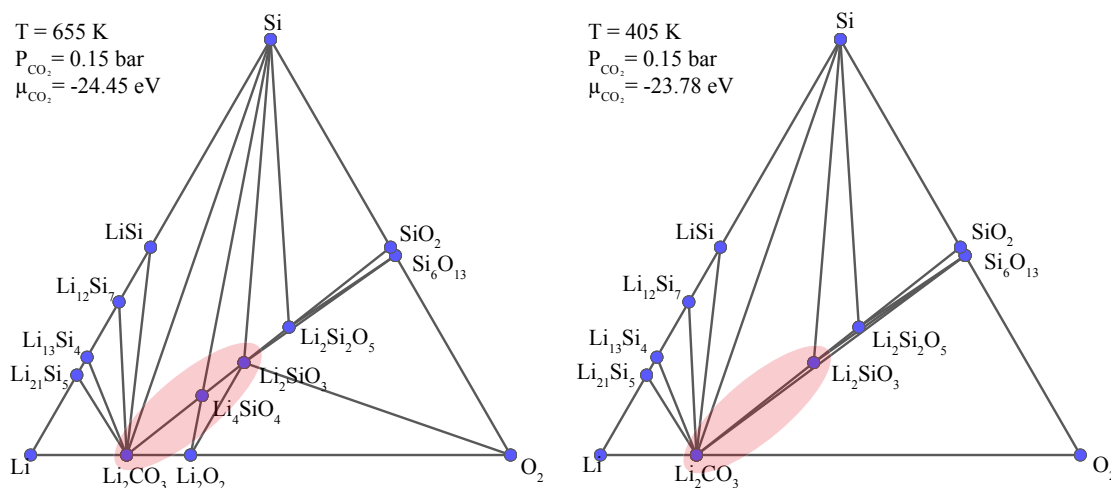
Figure 1: Ternary Li-Si-O phase diagrams under different \mu_{\text{CO}_2} obtained by applying the \text{CO}_2 grand potential to the Materials Project database. The physical equivalent of increasing the chemical potential is either an isothermal reaction performed with increasing p_{\text{CO}_2} , or an isobaric reaction under decreasing temperature. Vertices that are present in the lefthand phase diagram but are not present in righthand phase diagram represent phases which have decomposed as a result of the change in \mu_{\text{CO}_2} . The product phases of this decomposition reaction with \text{CO}_2 are situated at the vertices at either end of the edge where the original phase was formerly located. For example, \text{Li}_4\text{SiO}_4 transforms to a mixture of \text{Li}_2\text{CO}_3 and \text{Li}_2\text{SiO}_3 with increasing \mu_{\text{CO}_2} (see pink shaded area of the phase diagram).
