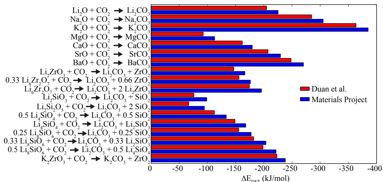
Figure 3: Comparison between the calculated \Delta E_{DFT} for this work (blue), and with the studies of Duan et al. (red). 19,20,23,38 There is a small but constant difference between the two studies, with the Materials Project \Delta E_{DFT} being 21 \text{ kJ mol}^{-1}_{\text{CO}_2} lower than the previous study on average.
