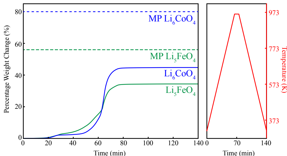
Figure 8: TGA traces for \text{Li}_5\text{FeO}_4 and \text{Li}_6\text{CoO}_4 under p_{\text{CO}_2} \approx 0.1 bar.
