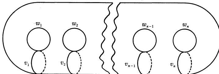
Figure 1. The canonical Heegaard diagram of S^3 of genus n , (1_n)
