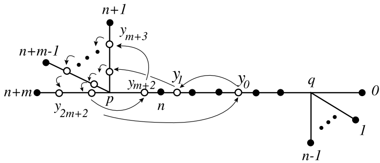
Fig. 12. Symbol \circ indicates the periodic orbit of y_0 , and \bullet is a vertex of (G^{\text{red}}_{m,n})_s . Note that y_0 \in e(q, n)^3 , y_1 \in e(q, n)^5 .
