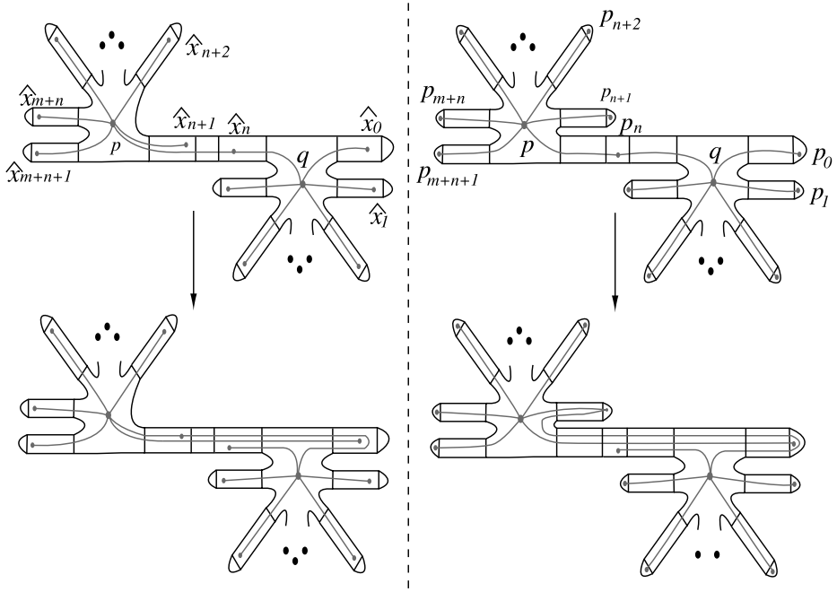
Fig. 11. Image of \hat{G} under g_{m,n} (left), image of G^{\text{red}}_{m+1,n} under g_{m+1,n} (right).
