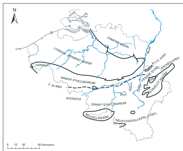
Figure 1. Location map of the studied areas. B.V.D. = Booze – Le Val Dieu High
