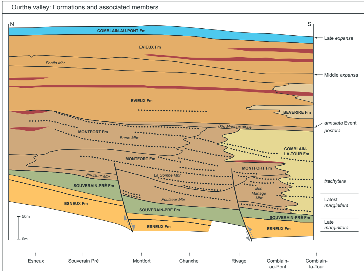
Figure 5. Lithostratigraphical scheme (after a palinspastic reconstruction of about 18 km) of the Condroz Sandstone Group in the “classical” Ourthe valley (S of Liège). This section extends from the town of Esneux in the N to the town of Comblain-la-Tour in the S. Black dotted lines represent conspicuous ball-and-pillow levels (“pseudonodules”). Thick red lines correspond to red beds.
