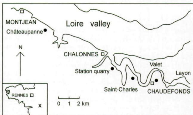
Fig. 1 – Location map of the quarries concerned by this paper at Montjean, Chalonnnes and Chaudéfonds in the southeastern Armorican Massif.
