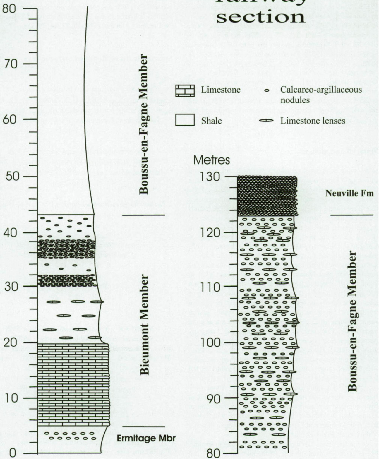
Fig. 2 — Lithological column of the upper part of the Moulin Liénaux Formation (Ermitage Member) and of the Grands Breux Formation (Bieumont Member and Boussu-en-Fagne Member). For the position of samples, see tables where their height from the bases of members is indicated.
