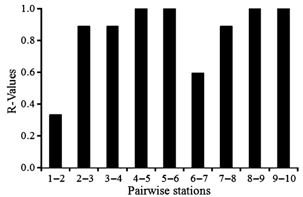
Fig. 6. r-Values resulting from ANOSIM pairwise tests for neighbour stations. Odd numbers = runnels, even numbers = sandbars. r > 0.5 indicates a clear separation between pairs of neighbour stations.
