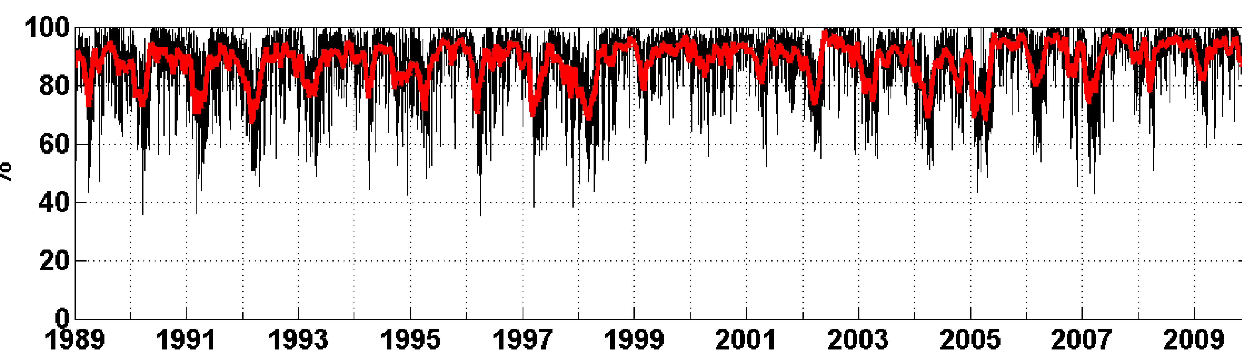
Figure 1. Spatial (above) and temporal (below) variation of cloud cover over the South China Sea in 1989–2009. The percentage of missing data is high in summer, and especially from the equator to 5°N.
