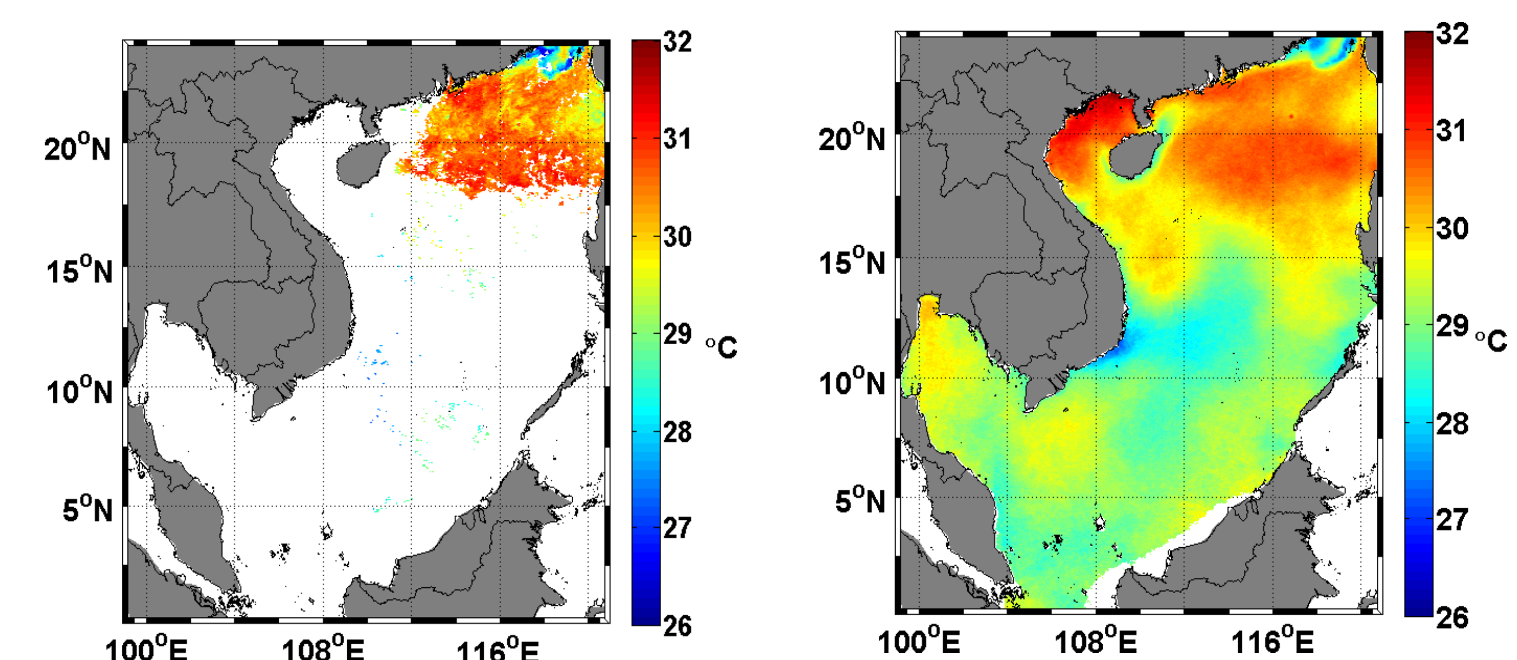
Figure 4. SST (right) was reconstructed by DINEOF from an image with cloud coverage 85.89% (left) on 28 August 2009. The reconstructed SST clearly shows the upwelling phenomena in the northeastern South China Sea and in the center of Vietnam in summer.
