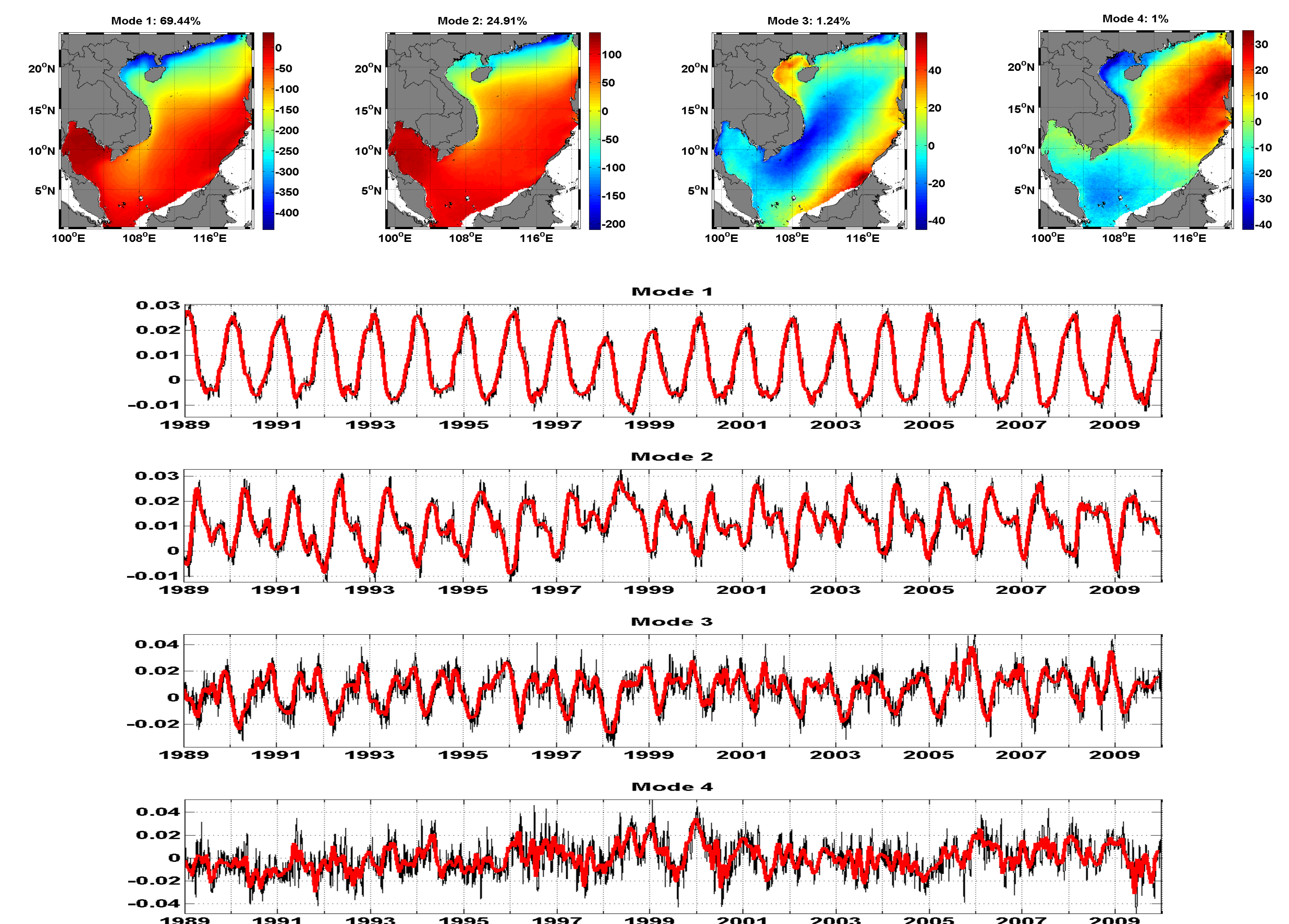
Figure 2. Spatial and temporal EOF of mode 1-4.
