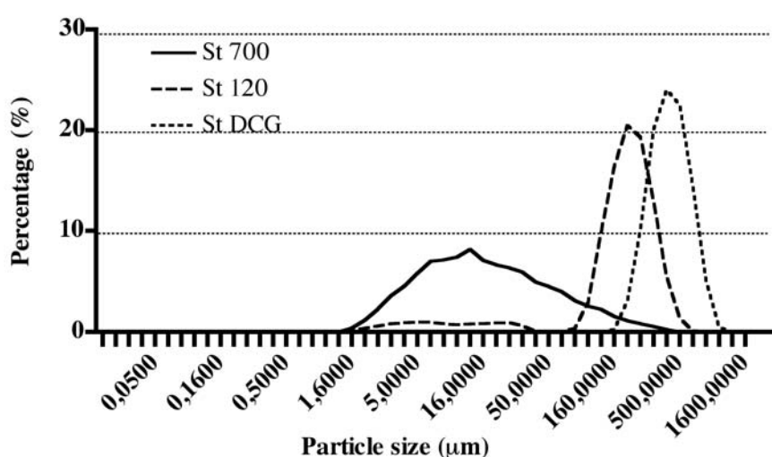
Figure 11. Particles size distribution as measured with a laser granulometer.
