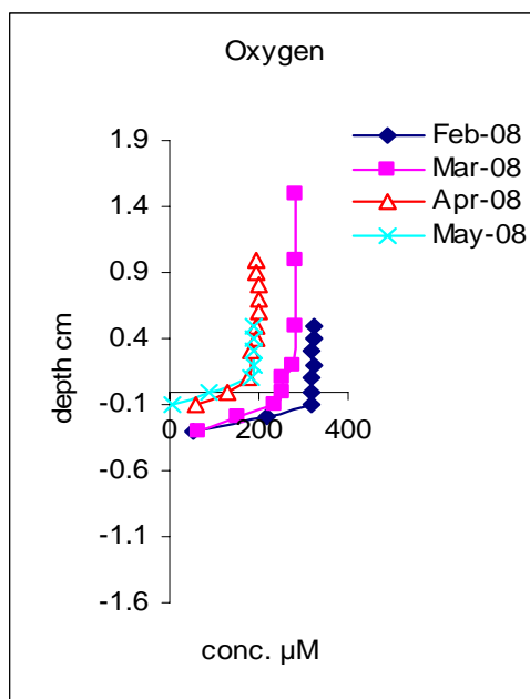
Figure 21. Oxygen concentration in sediments of station 130 (February to May 2008).
