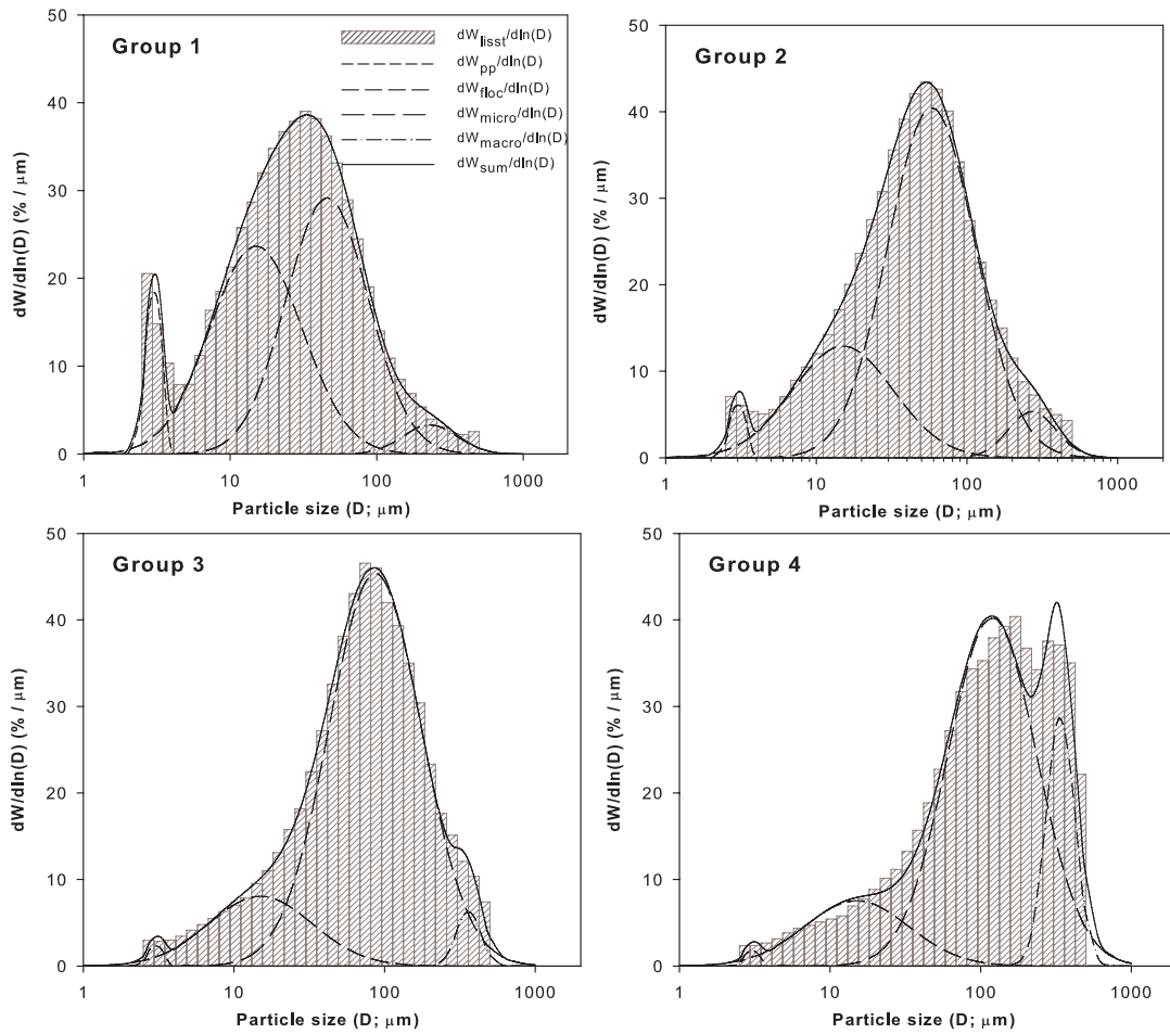
Figure 2.7: January–February and March–April 2008 deployments: averaged PSD for the four entropy groups, dW_{\text{lisst}}/d\ln(D) , together with the fitted sum of the four log-normal functions, dW/d\ln(D) .
