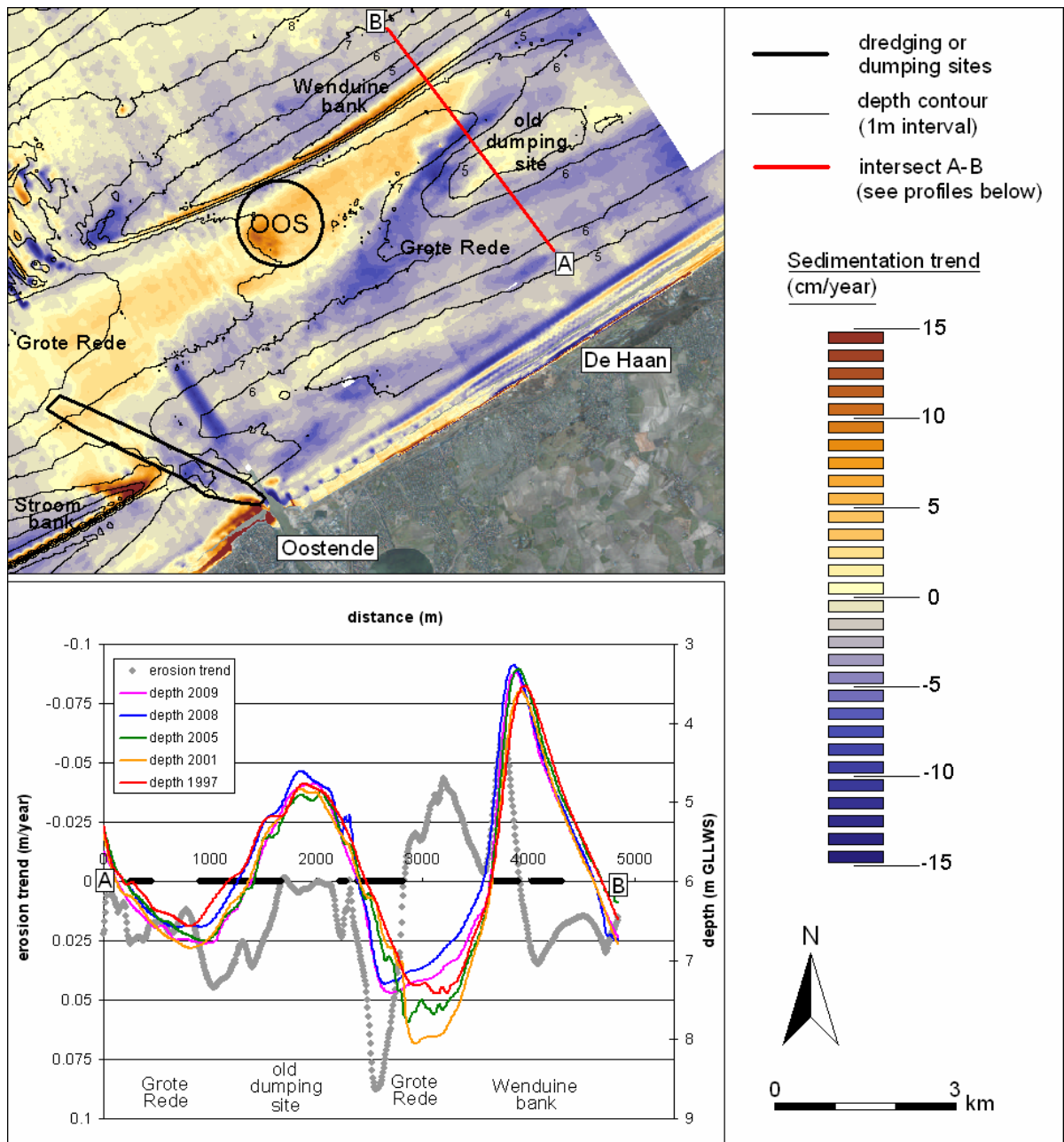
Figure 4.2: Top figure: erosion-sedimentation trend for beach, foreshore and the nearshore between Oostende and De Haan. Bottom figure: depth profiles (solid lines, right vertical axis) and erosion trend profile (dotted line, left vertical axis) along cross section A-B.
