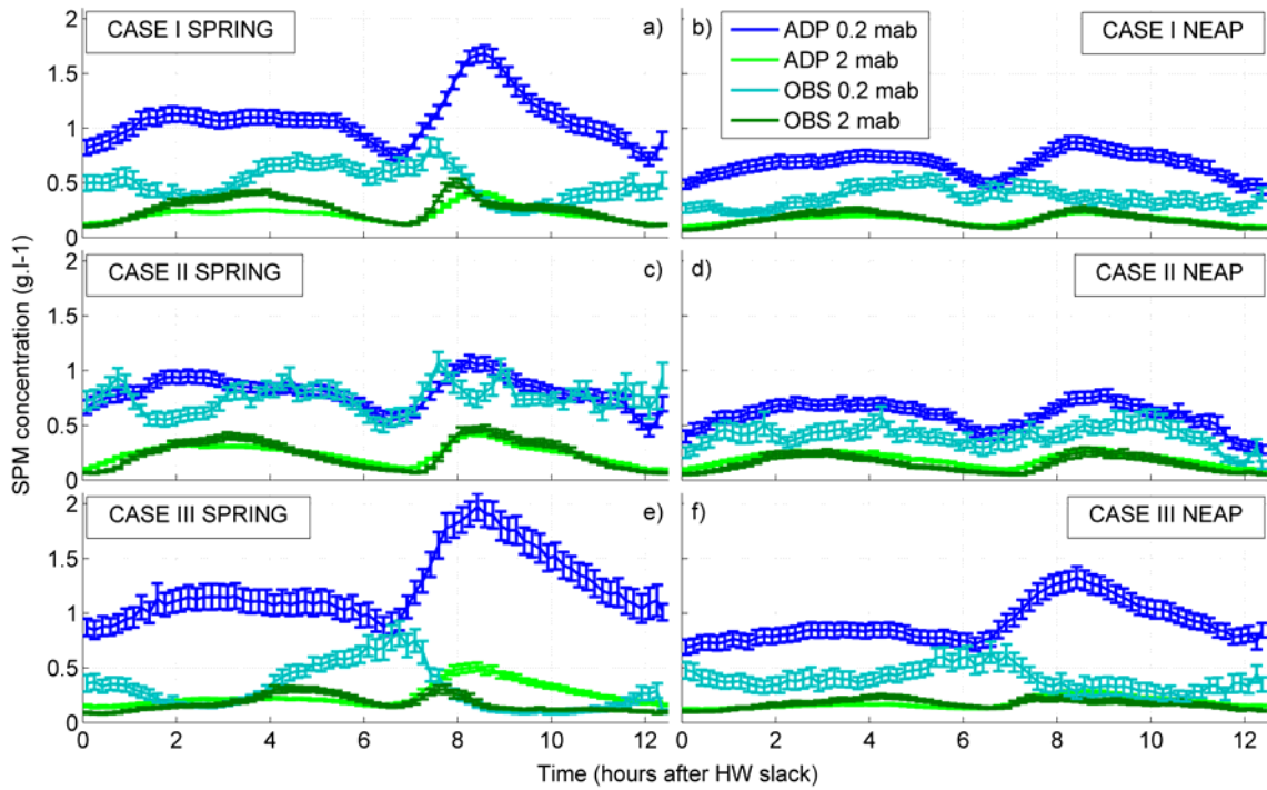
Figure 2.4: Ensemble-averages of tidally varying SPM estimates from OBS and ADP at 0.2 (blue) and 2 mab (green). The error bars indicate standard error. (Case I: no wind, case II: NW-NE wind, case III: SW wind).
