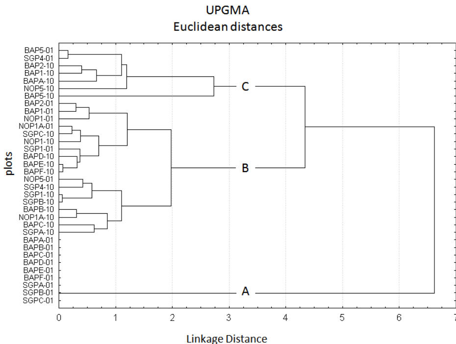
Figure 6. Cluster analysis, considering mean height and log-transformed tree density values, from permanent plots located in the southern sector. Plot code followed by 01 and 10 corresponding to data collection from 2001 and 2010 respectively. Group A indicates plots absent in 2001; Group B indicates mangrove forests with intermediate structural development, and Group C mangrove forests with high structural development.
