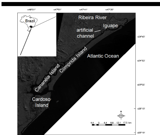
Figure 1. Study area location, the Cananéia-Iguape Coastal System (CICS), on the southern coast of the State of São Paulo, Brazil. Georeferenced Landsat TM5 band 4, from path/rows 219/77 and 220/77, from 17/06/1997 and 24/06/1977, respectively.
