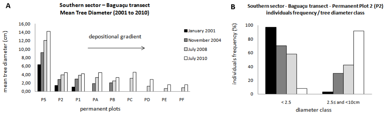
Figure 5. Structural development of mangrove vegetation between January 2001 and July 2010 in permanent plots located along transects in the southern sector. A. Mean tree diameter values, of permanent plots, along the depositional gradient, over the monitored period. B. Individuals frequency of tree diameter classes, from permanent plot 2 (P2), indicating mangrove plant growth, over time.
