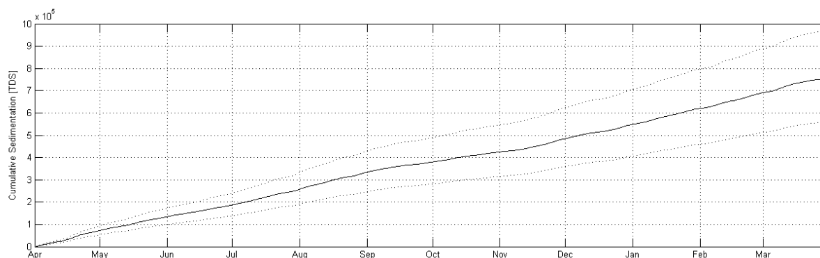
Figure 5-21: Cumulative natural sedimentation in black (x100,000 TDS) with zero at April 1 st 2007, uncertainty band in grey. Average sedimentation rate varies with seasons, lowest rates in September and October.
