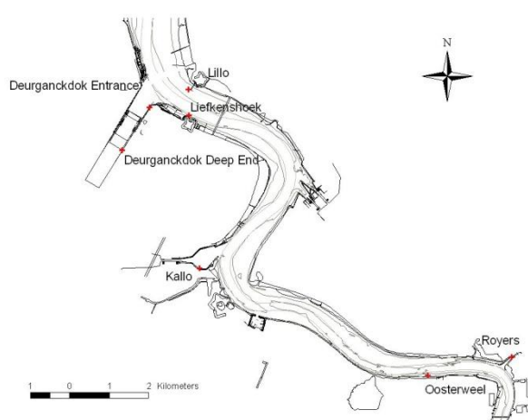
Figure 3-11: Calibration measurements - 23/06/2006 & 18/09/2006
