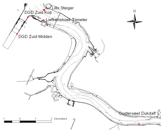
Figure 3-10: Calibration measurements - 15/03/2006 & 14/04/2006
