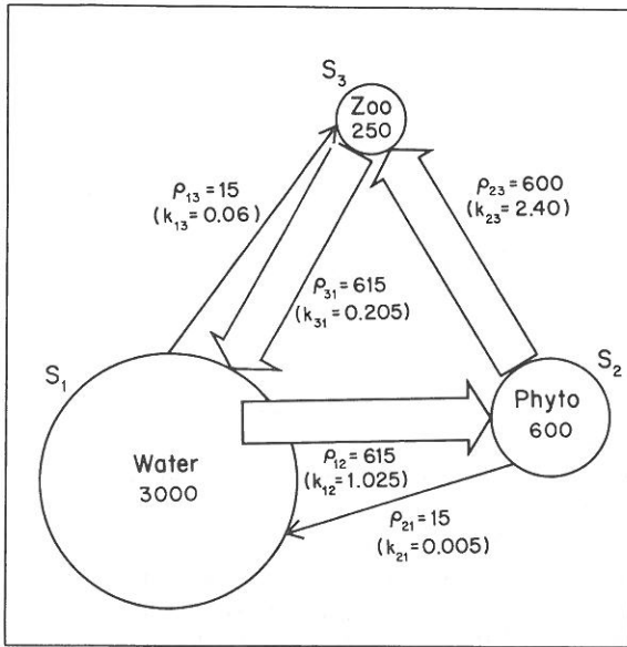
Fig. 1. The three-compartment, closed, steady-state model of CONOVER & FRANCIS (1973) involving water, phytoplankton and zooplankton. Numerical values for stocks (s), rate constants (k) and flows ( \rho ) as used in an example by CONOVER & FRANCIS. We assumed that these stocks and flows are expressed in \mu\text{g C/l} and \mu\text{g C/l/day} respectively.
