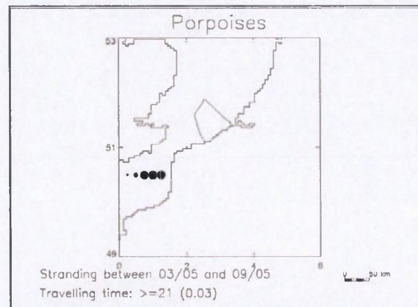
Figures 4 and 5: Modelling as for figures 2 and 3, but now the travelling time of the particles is between 14 and 21 days (above left and right) and greater than 21 days (below left and right)..
