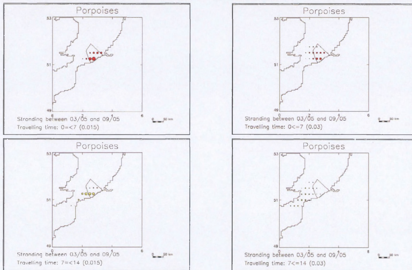
Figures 2 and 3: Particles that reached the coast in less than 7 days (above left and right), and between 7 and 14 days (below left and right). The circles indicate the release positions of the particles. The radius of each circle is roughly proportional to the number of particles released from that point that reach the coast. The results obtained with a wind drift factor set equal to 0.015 are shown in the left panels. Those obtained with a wind drift factor set equal to 0.03 are shown in the right panels.
