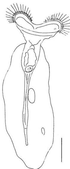
Fig. 44. Collothecacean rotifer: Collothecha mutabilis . Scale bar = 50 \mu m.
