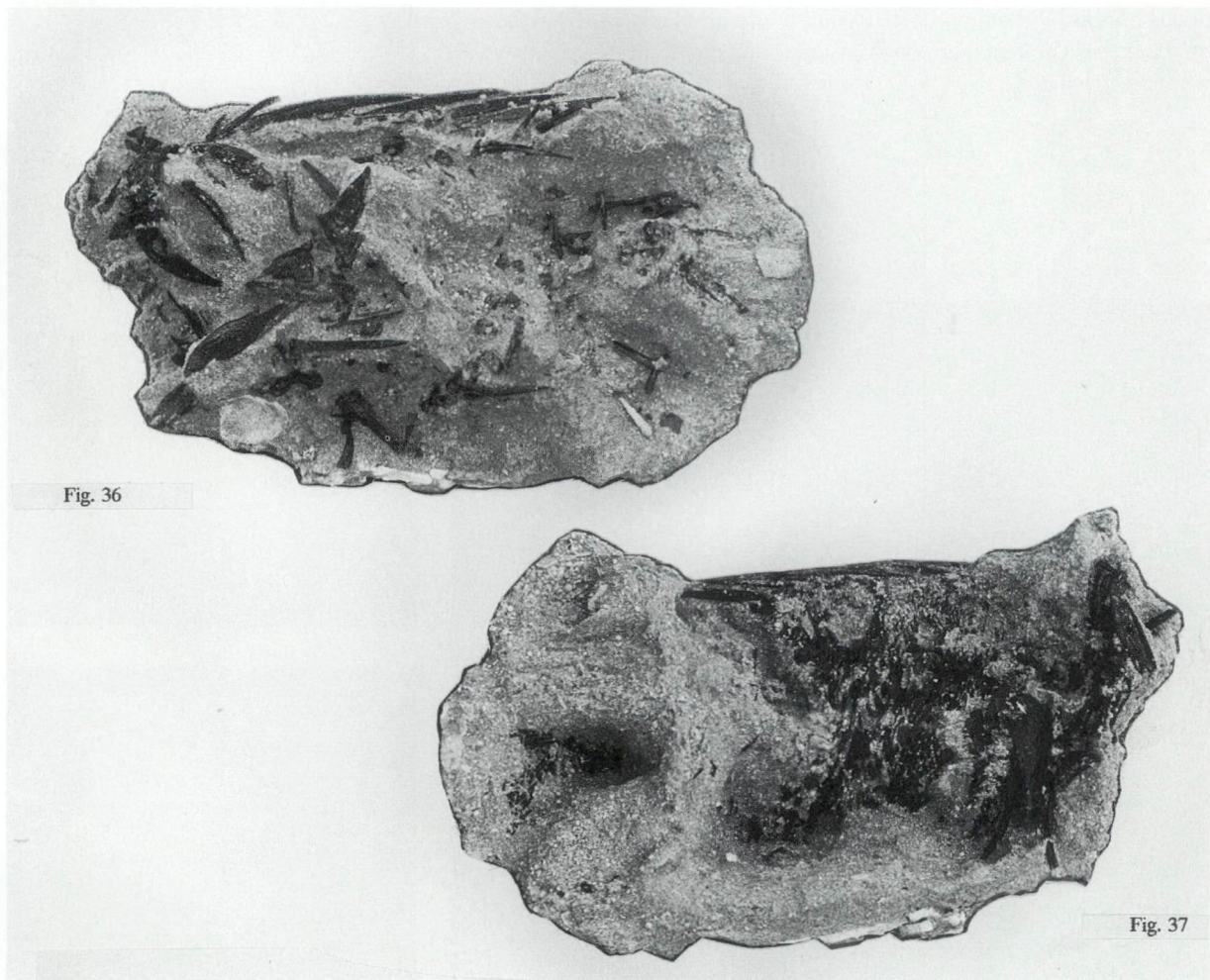
Figs. 36 and 37: A fish of the family Priacanthidae (Percomorphii), burrowed in a Nautilus conch at Meldert.
