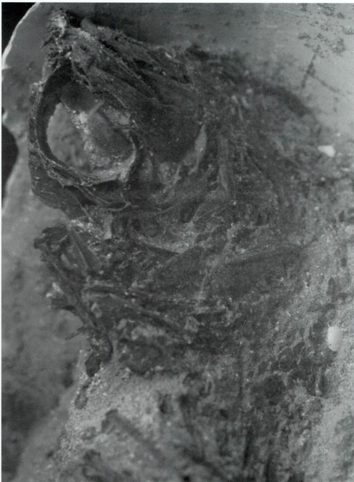
Fig. 38: A Priacanthid fish in dead position with all bones in connection, found in a Nautilus conch in the sandpit Verlee at Balegem (East-Flanders) in the Sands of Lede. This unique specimen was discovered by M. René Lardinois and delicately disengaged from its sandy gangue by M. Georges Wouters.
