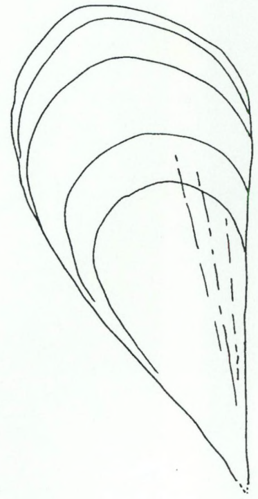
Fig. 123 Fossil Atrina nov.sp. Kallo, Pliocene, Belgium
