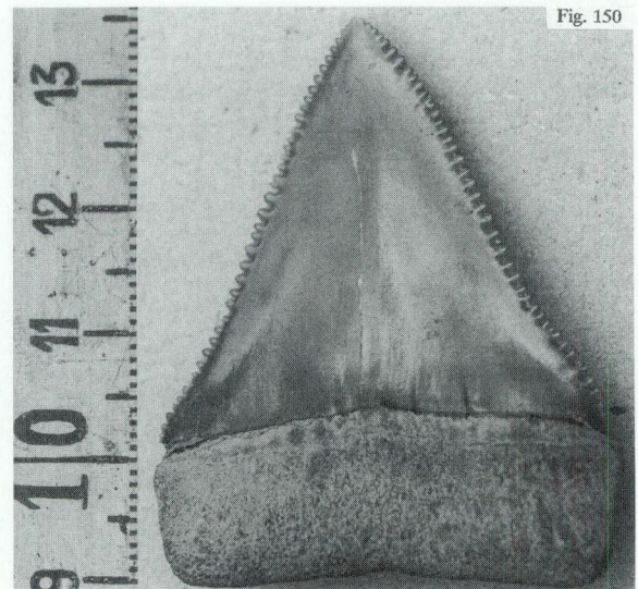
Fig. 150: Carcharodon carcharias (formerly rondeleti ) Vrasenedok, Kallo.
