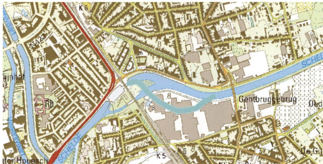
Figuur 3.76 Rechttrekking aan de stuw in Gent / Canalization near the present dam in Gent
