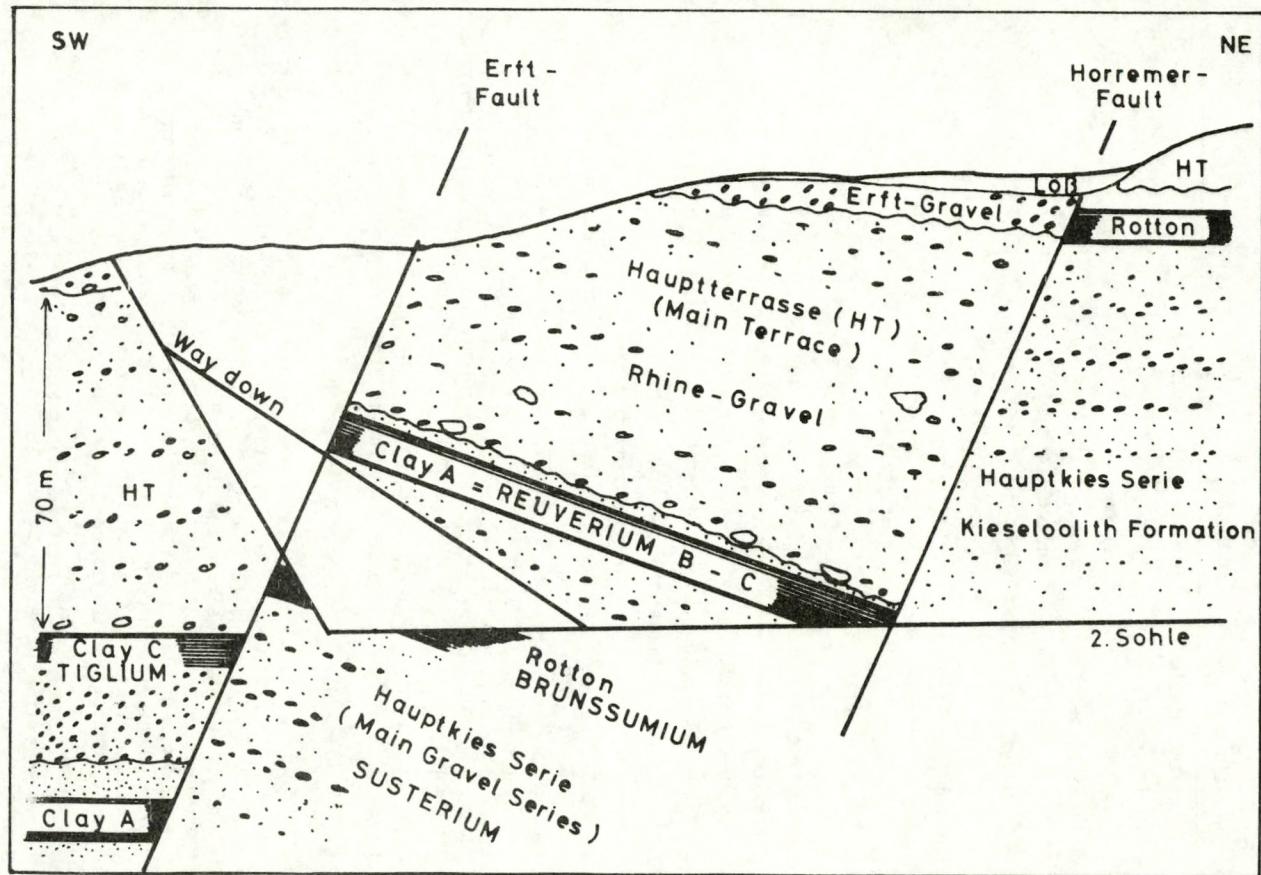
Fig. 12 - THE TERTIARY AND QUATERNARY DEPOSITS IN THE BROWN COAL MINE AT FRECHEN, LOWER RHINE BASIN
