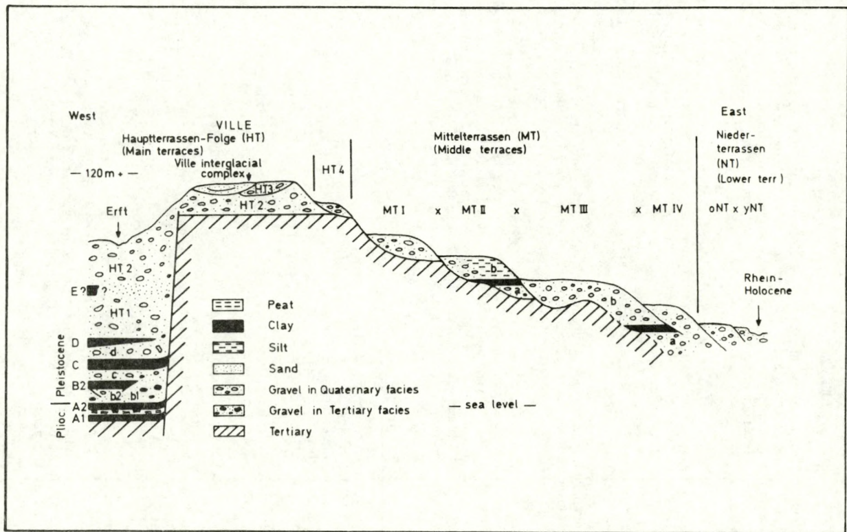
Fig. 13 - SCHEMATIC SECTION OF THE 'JUNG' TERTIARY AND QUATERNARY IN THE SOUTHERN LOWER RHINE BASIN
