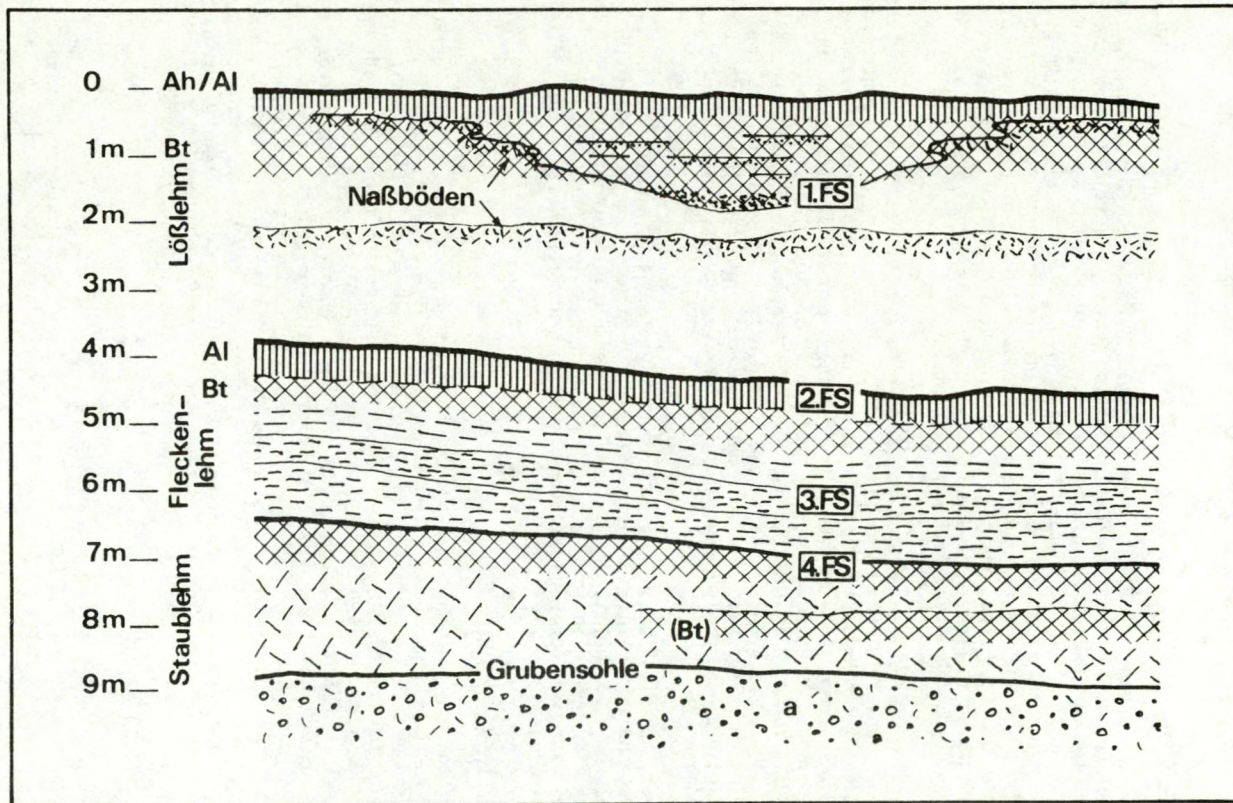
Fig. 15 - BRICKWORKS SECTIONS AT RHEINDAHLEN, LOWER RHINE BASIN
