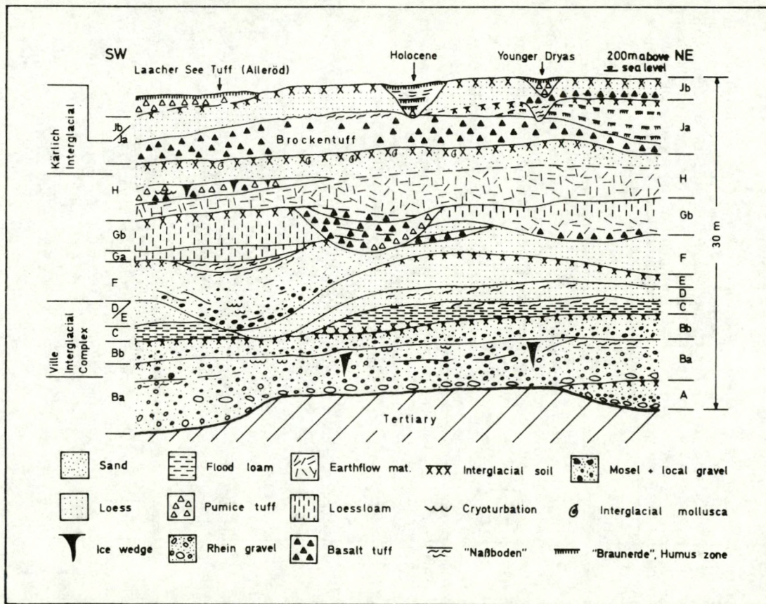
Fig. 10 - SECTION AT KARLICH, NEUWIEDER BASIN
