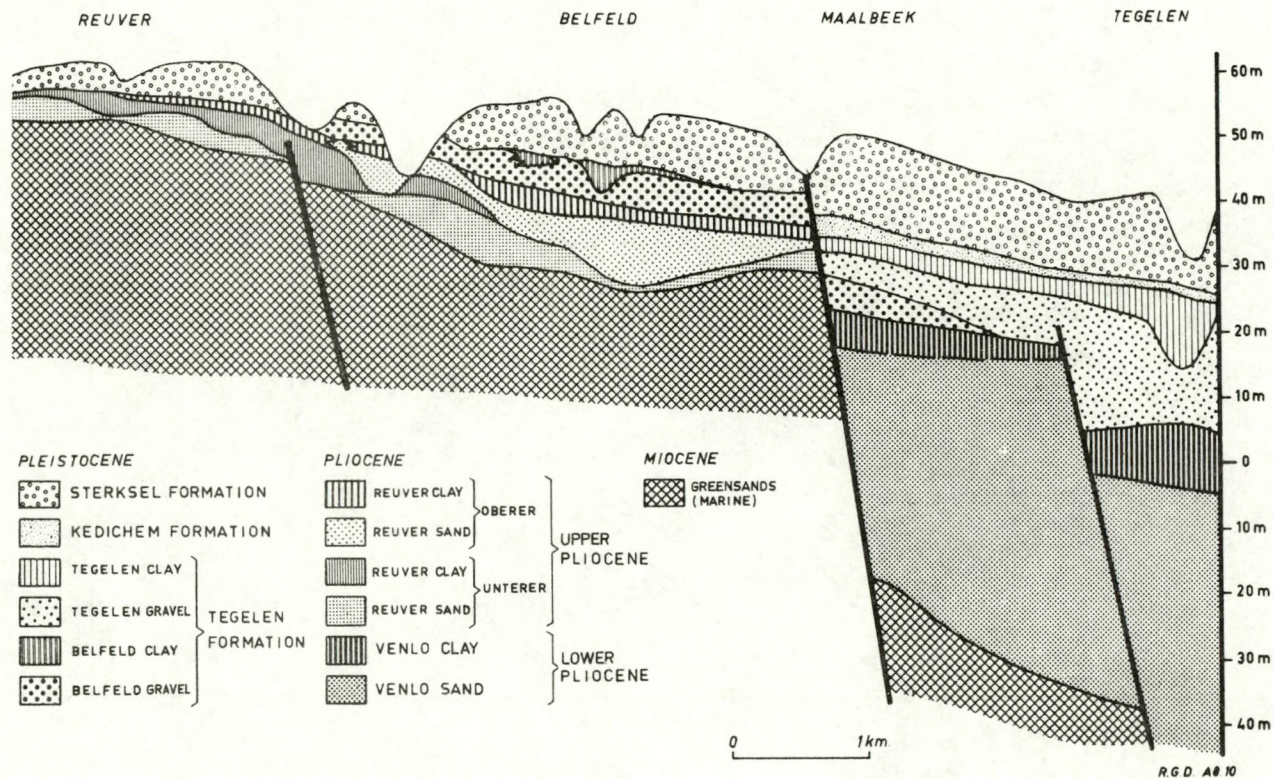
Fig. 17 - SECTION OF THE REUVER-TEGELEN AREA LOCATION
