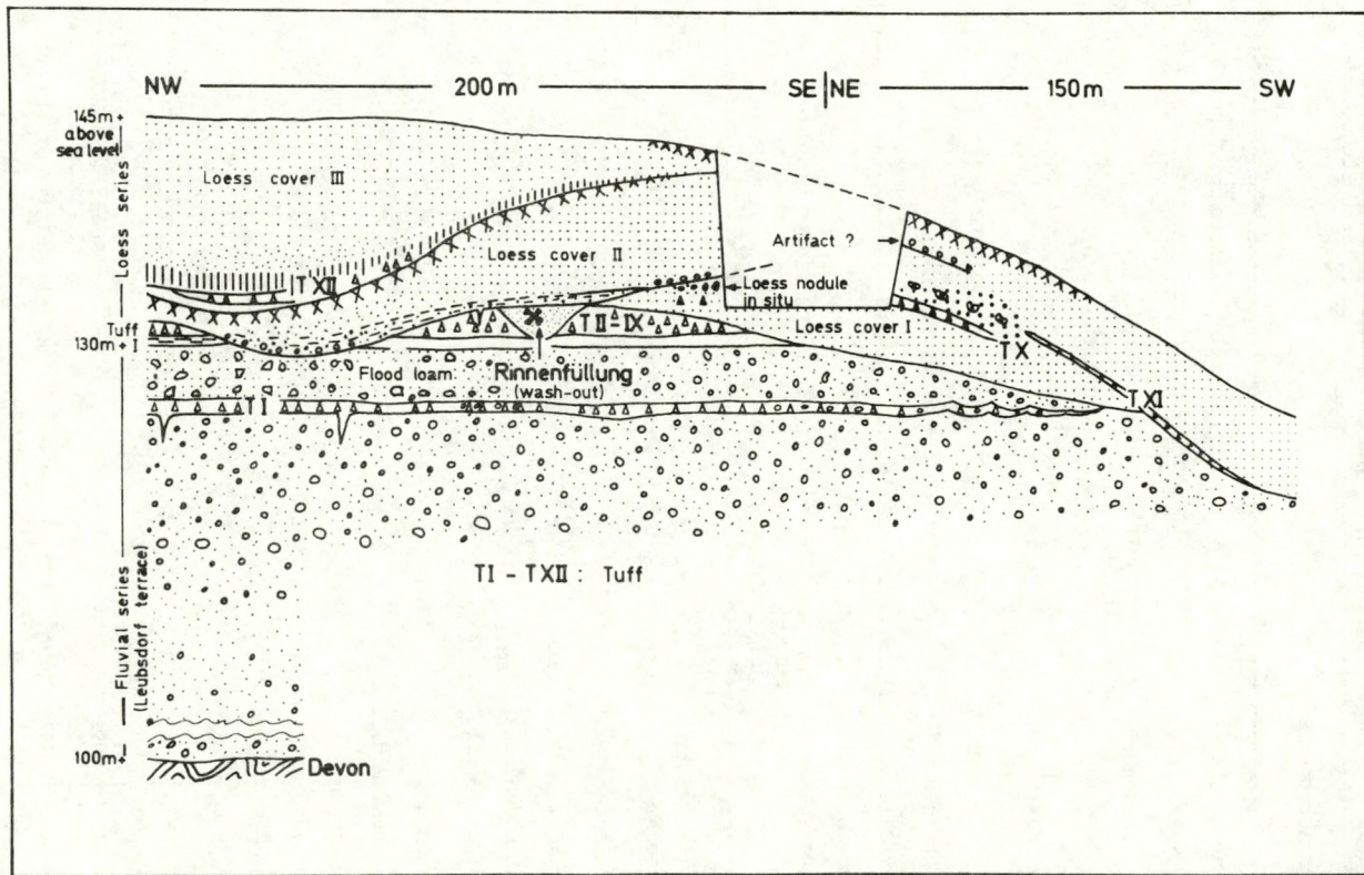
Fig. 11 - THE SECTION AT ARIENDORF, LOWER MIDDLE RHINE
