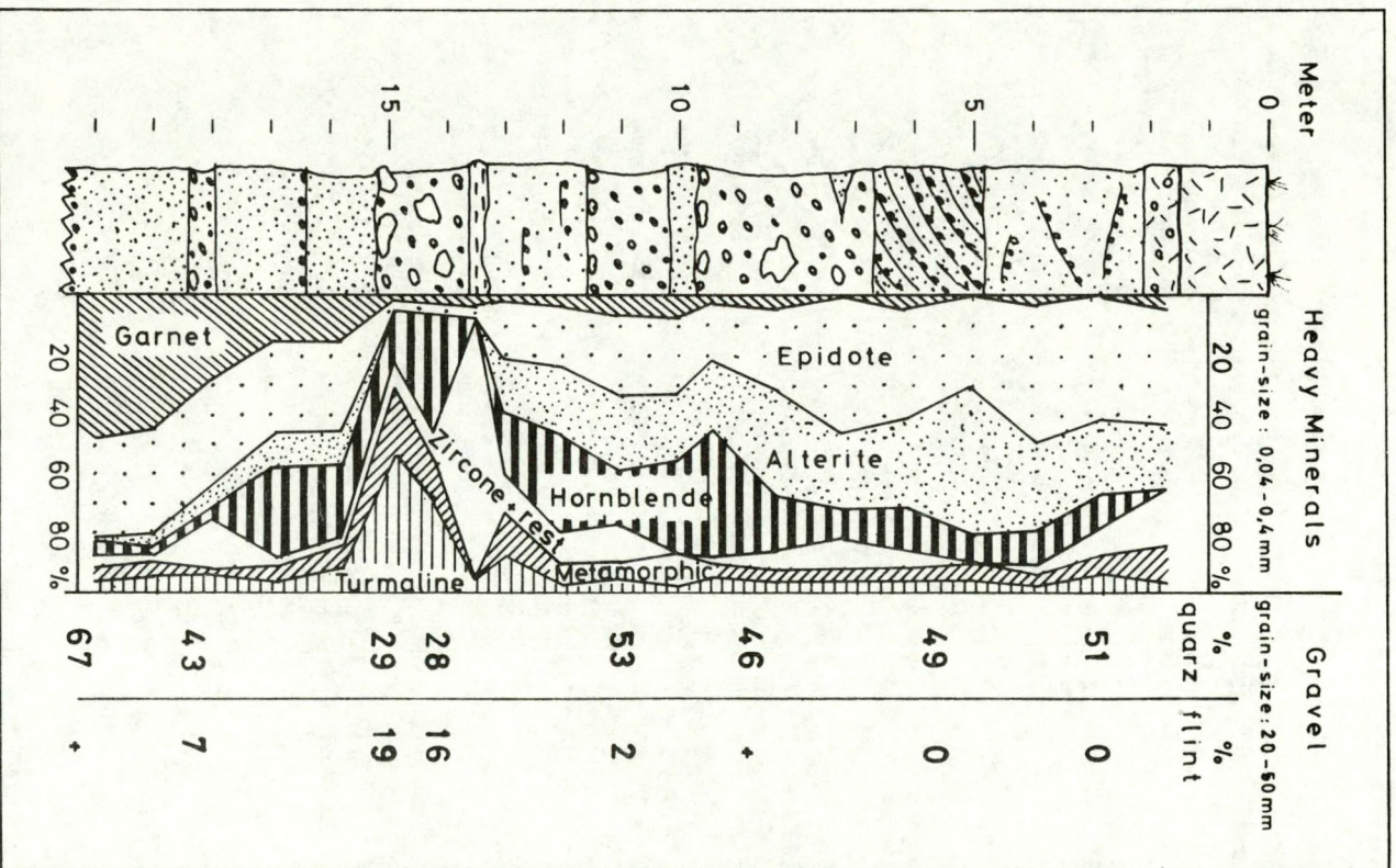
Fig. 14 - ALTERNATING RHINE AND MEUSE GRAVELS IN THE EARLY QUATERNARY AT HOLZWEILER, LOWER RHINE BASIN
