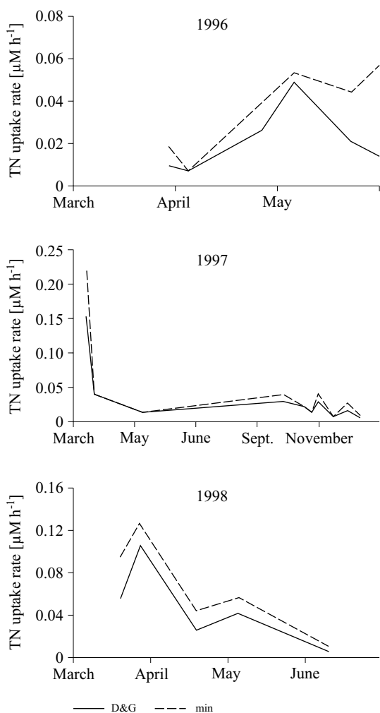
Fig. 3. Trends of TN uptake rates calculated using Dugdale & Goering's model (D&G) and minimum estimates from Elskens' model
