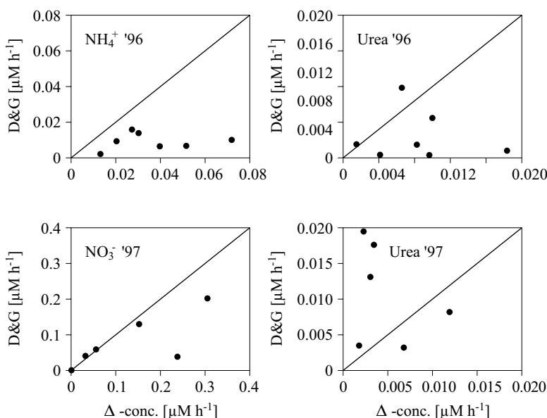
Fig. 1. Scatter plot of some of the observed divergence in the uptake rates derived from Dugdale & Goering's (D&G) and those derived from the differences between the initial and final concentrations of the nutrients ( \Delta -conc.) during incubation. The bisect lines indicate the expected linearity of the data sets
