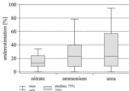
Fig. 4. Deviations of uptake rates calculated by the D&G equation from the minimum estimates of the model by Elskens et al. (2002)
