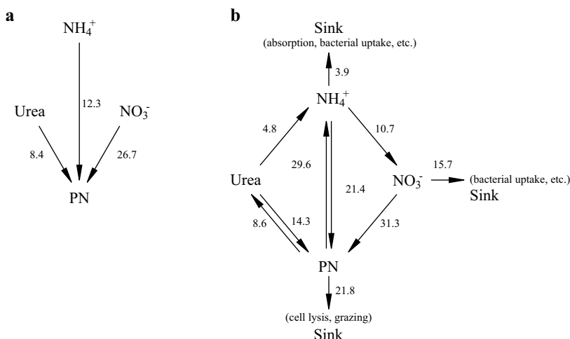
Fig. 7. Comparison of nitrogen flux rates as estimated from the equation of (a) Dugdale & Goering (1967) and (b) the Elskens model (2002). Nitrogen flux rates are presented as mean estimated values expressed in \text{nM h}^{-1}
