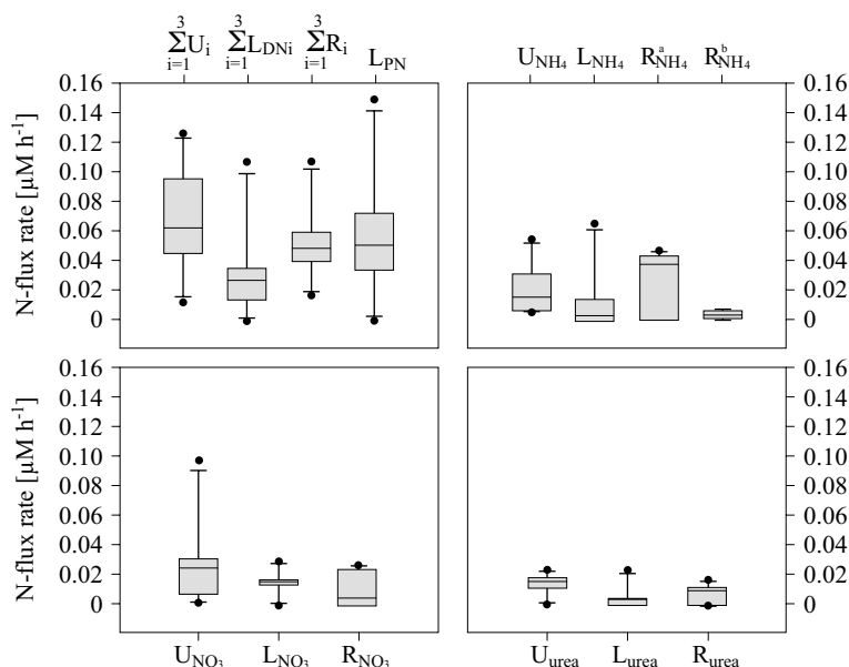
Fig. 6. Box and whisker plots of N-flux rates for 1998 from the Elskens model approach. The values correspond to the minimum estimates of the model. U_{\text{NH}_4} , U_{\text{NO}_3} and U_{\text{urea}} – corresponding nutrient uptake rates; L_{\text{NH}_4} , L_{\text{NO}_3} and L_{\text{urea}} – corresponding nutrient loss rates; L_{\text{PN}} – loss rate of PN; R_{\text{NO}_3} and R_{\text{urea}} – corresponding nutrient regeneration rates; R_{\text{NH}_4}^{\text{a}} – ammonium regeneration estimated by Lancelot & Billen’s model; R_{\text{NH}_4}^{\text{b}} – ammonium regeneration estimated by Elskens’ model; \sum_{i=1}^3 U_i , \sum_{i=1}^3 L_{\text{DN}_i} and \sum_{i=1}^3 R_i – sum of uptake, loss and regeneration rates of the three nutrients
