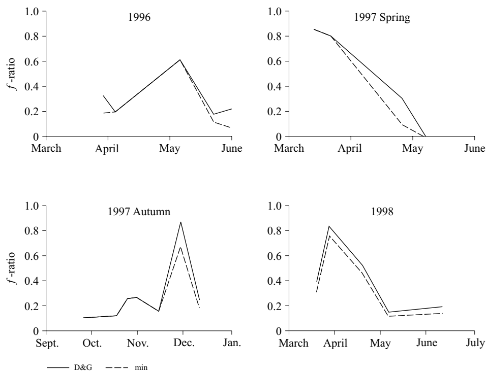
Fig. 5. Comparison of f -ratios and variations for the uptake rates calculated by the D&G model and for the minimum estimated uptake rates obtained using Elskens' model
