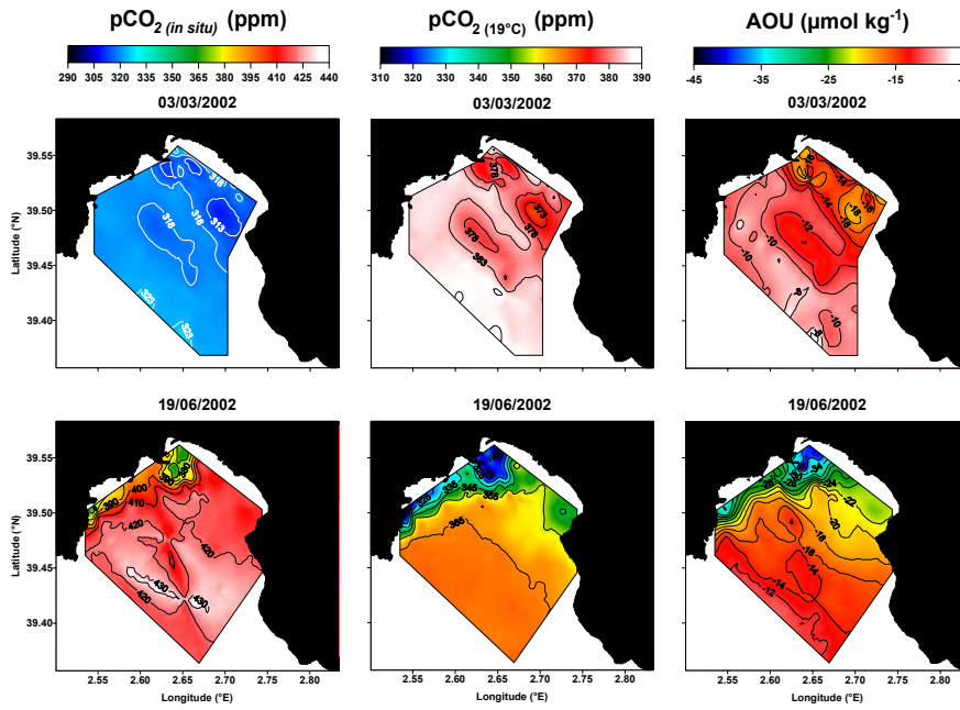
Fig. 8. Surface distributions of p\text{CO}_2(\text{in situ}) (ppm), p\text{CO}_2 normalized to a constant temperature ( p\text{CO}_2(19^\circ\text{C}) , ppm) and \text{AOU} ( \mu\text{mol kg}^{-1} ) obtained on 3 March 2002 (EUBAL-I cruise) and 19 June 2002 (EUBAL-II cruise).
