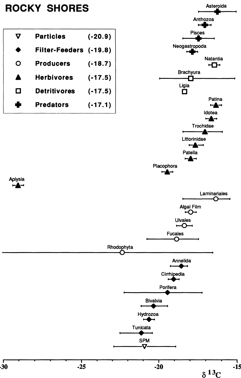
Figure 4. Distribution of δ 13 C values (means and absolute deviations) of the main systematic groups (according to trophic guild) encountered on rocky shores. SPM: suspended particulate matter. Overall values are given in the frame.
