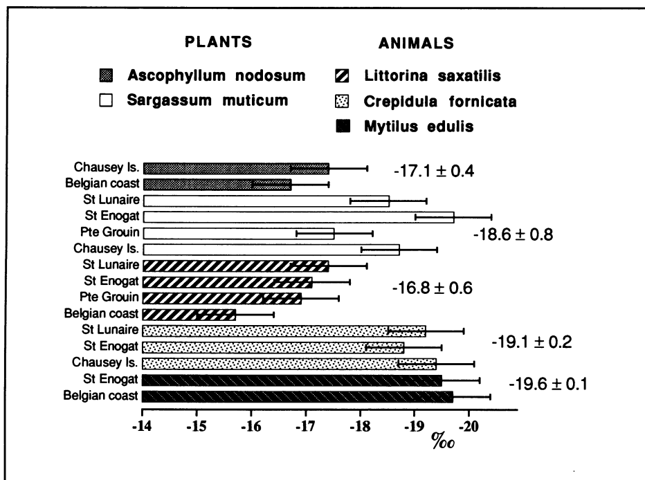
Figure 3. Geographical variability in the δ 13 C of different common species. For each of them, bars are arranged from western to eastern sampling sites. Error lines refer to mass spectrometer accuracy.
