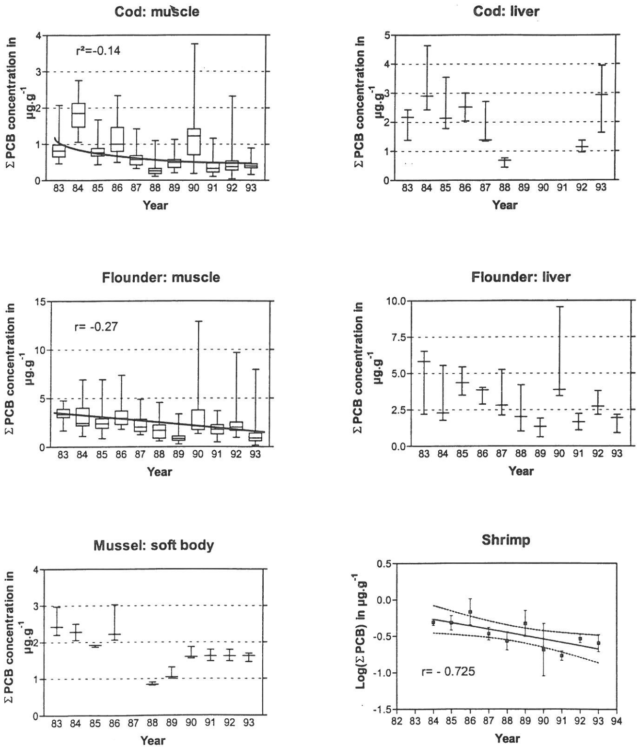
Figure 6: ΣPCB concentrations in µg/g fat weight for cod, flounder and mussel (lines illustrate calculated significant trends; r , correlation coefficient; boxes, median and 25 and 75 percentiles; whiskers, minimum and maximum) and linear trend for the \text{Log}(\Sigma\text{PCB}) concentration in shrimp ( r , correlation coefficient; dotted line, 95 % of the mean).
