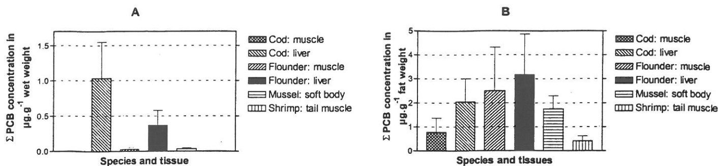
Figure 3: PCB concentrations for cod, flounder, mussel and shrimp, (A) not normalised and (B) normalised on total lipid content.
