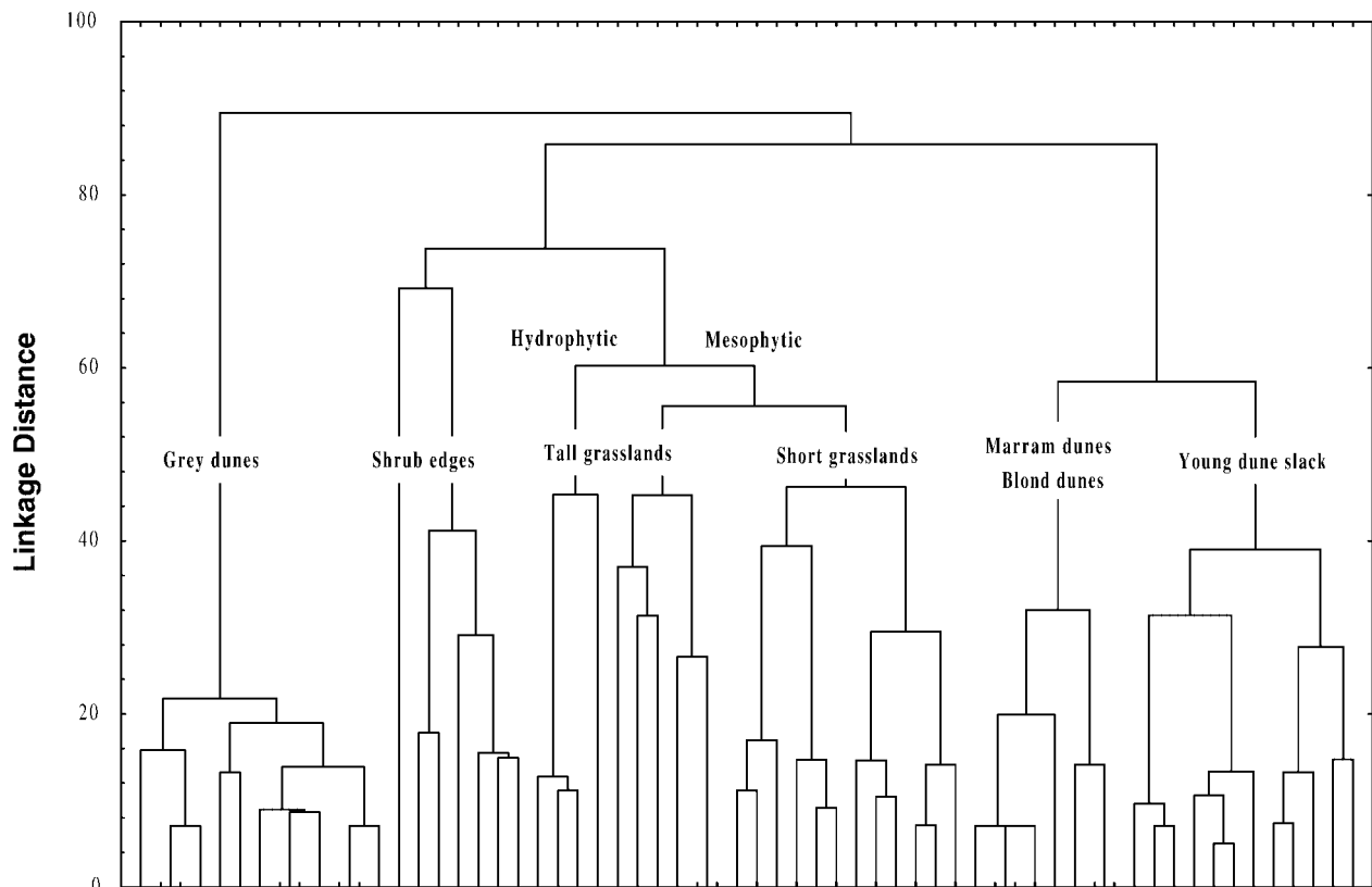
Fig 3. – Bray Curtis similarity dendrogram of the vegetation composition around the pitfall traps with P. monticola .
