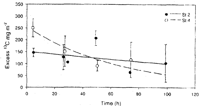
Fig. 4. Excess ^{13}\text{C} inventory as a function of time. Exponential fits with attenuation coefficients of -0.0052 \pm 0.005 (Sta. 2) and -0.012 \pm 0.005 (Sta. 4) have been indicated as well. Error bars represent standard deviations.
