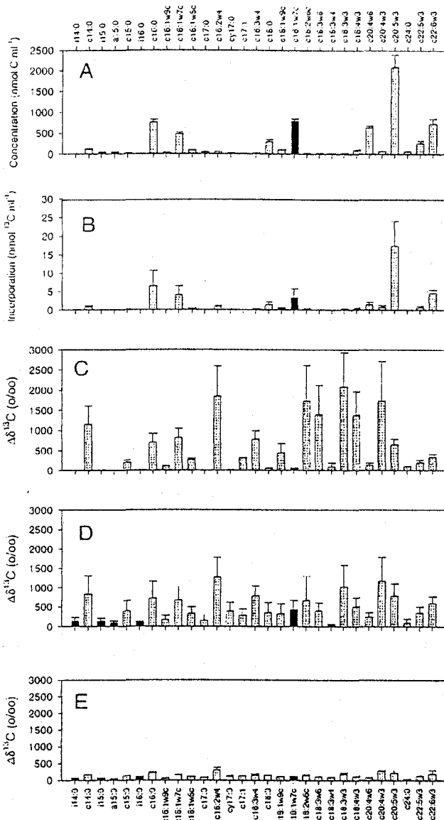
Fig. 6. (A) Concentrations of individual PLFA (4-h example). (B) 13 C incorporation in PLFA after 2 d. (C-E) Specific labeling patterns of PLFA ( \Delta\delta^{13}\text{C} ) after 4 h, 2 d, and 4 d. Error bars represent standard deviations. Solid bars show bacterial PLFA.
