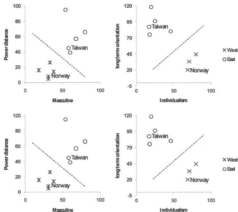
Fig. 1. A plot of Hofstede's cultural dimensions for north European countries (Norway, Sweden, Denmark, Finland and the Netherlands) and Confucian countries in South East Asia (Taiwan, China, Hong Kong, Japan and South Korea). The left plot shows the Masculine–Power distance plane and the Individuality–Long term orientation plane. Note that uncertainty avoidance is not plotted and that long term orientation data for Finland and Denmark were unavailable.
