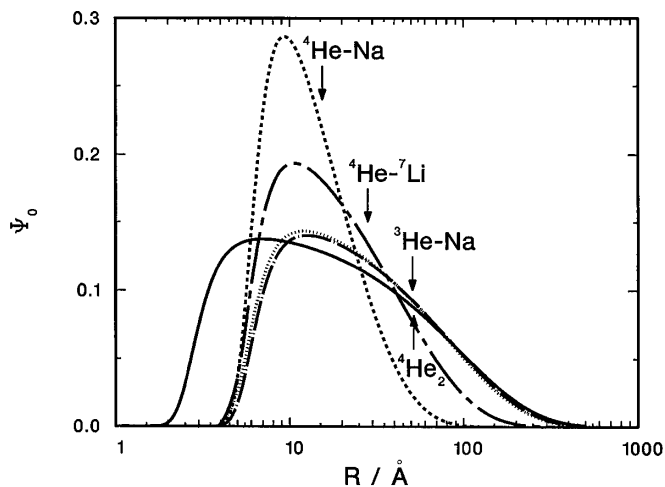
FIG. 1. Ground state wave functions for selected alkali-helium pairs from variational calculations on the KTTY potential without retardation. The 4 He- 6 Li wave function almost coincides with 3 He- 23 Na and is indicated by the thin dotted curve. Helium dimer (solid line) is shown for comparison. Arrows indicate \langle r \rangle expectation values. Note the logarithmic distance scale.
