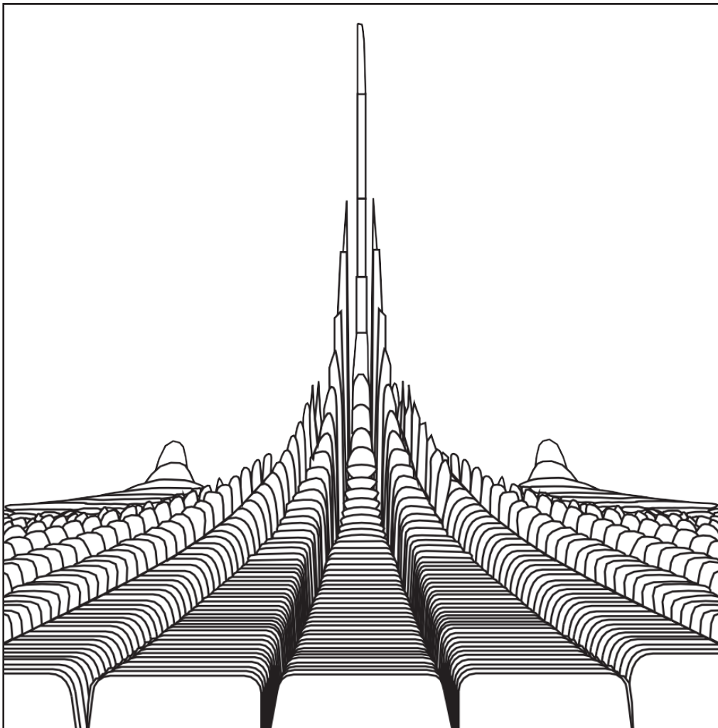
Figure 1 Quantum potential for two Gaussian slits
