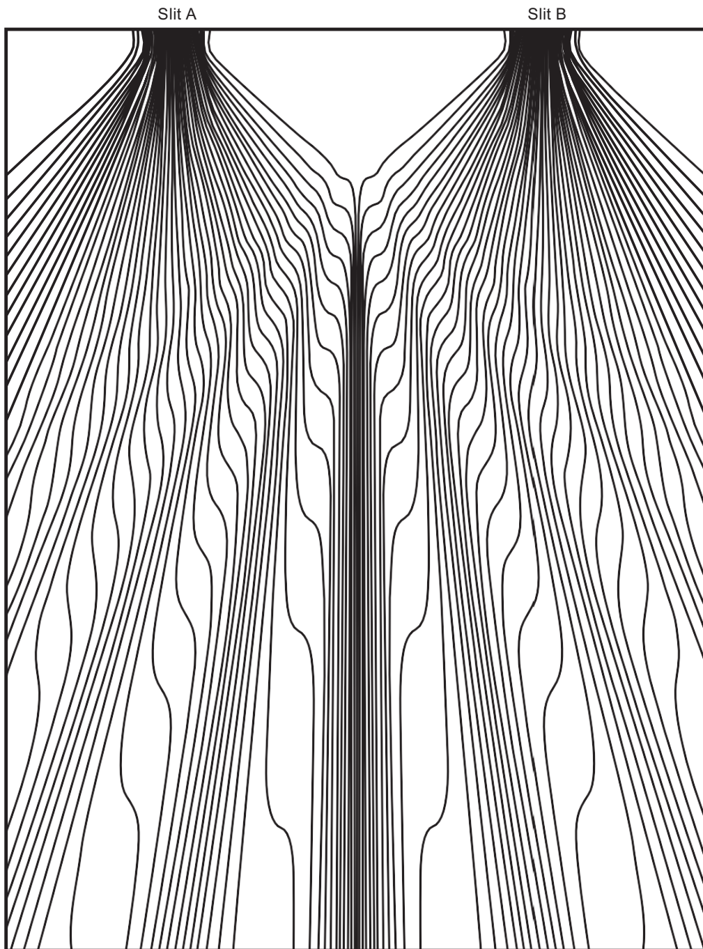
Figure 2 Trajectories for two Gaussian slits
