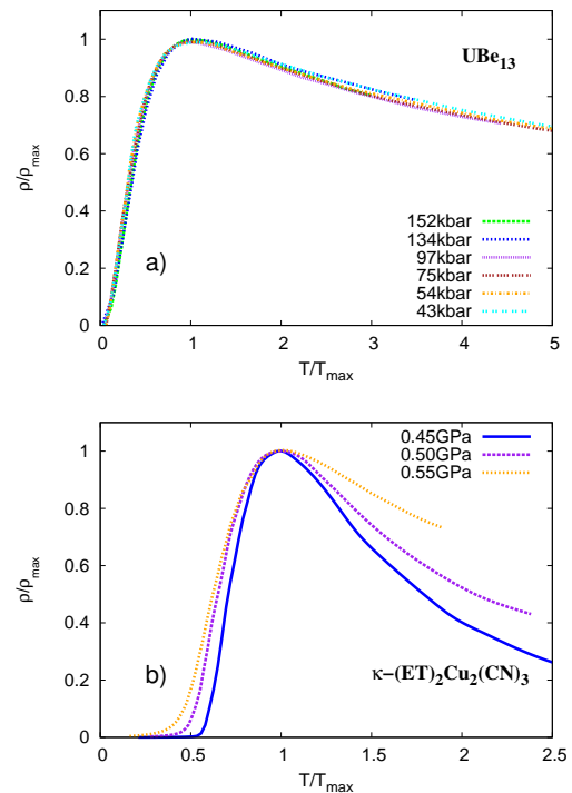
FIG. 6: (Color online) Scaled resistivity curves for UBe_{13} (a) and \kappa-(ET)_2Cu_2(CN)_3 (b), for different external pressure. The data are taken from Refs. 4 and 7.
