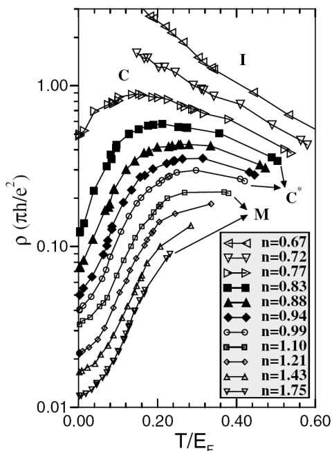
FIG. 1: Resistivity as a function of temperature from the experiments on Si MOSFET by Pudalov et al. (Ref. 19).
