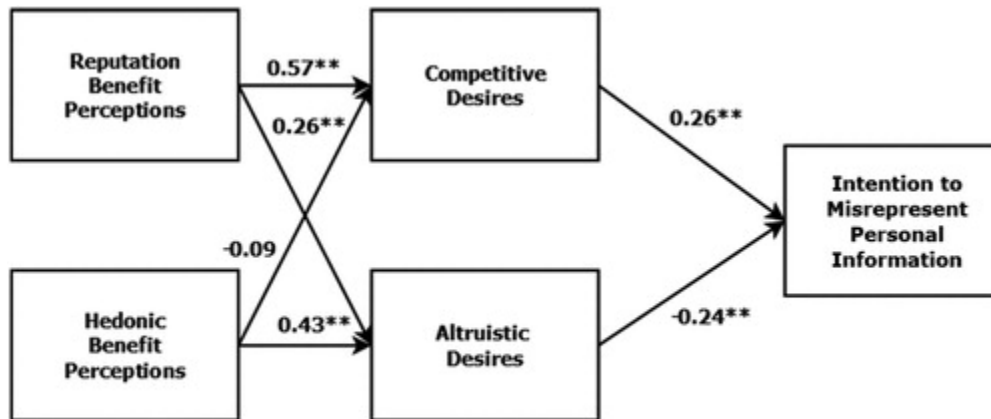
Figure 4. Results of structural equation modelling.
