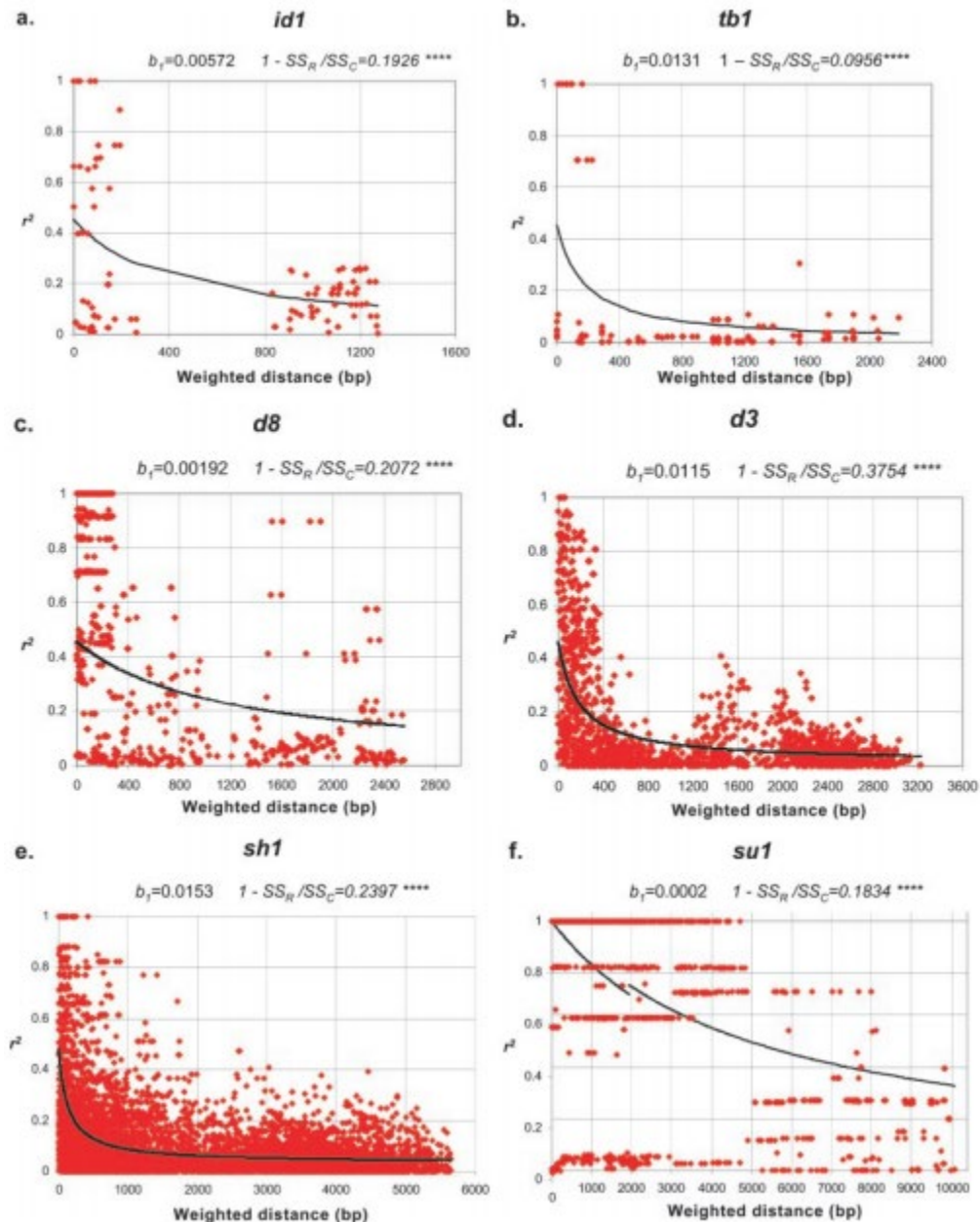
Figure 1. Plots of squared correlations of allele frequencies ( r^2 ) against weighted distance between polymorphic sites in six candidate genes: (a) id1 , (b) tb1 , (c) d8 , (d) d3 , (e) sh1 , and
