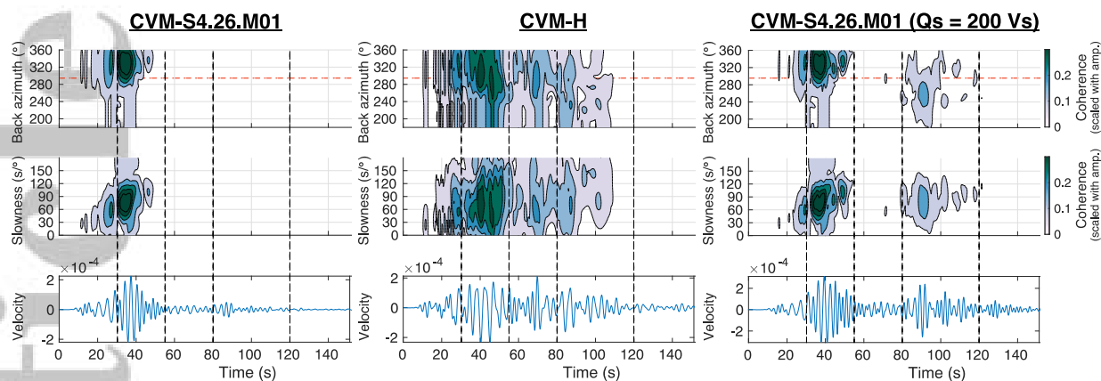
Figure 10. Plots show the back azimuth and slowness of P-, S- and surface wave synthetic arrivals from the Beverly Hills event at Santa Fe Springs (SFS) array generated using model CVM-S4.26.M01 ( Q_s = 50 V_s ), CVM-H and CVM-S4.26.M01 ( Q_s = 200 V_s ). The coherence is scaled with amplitude to highlight stronger shaking. The seismogram is bandpass filtered between 2 – 10 seconds with a two-pass Butterworth filter. The dashed lines indicate the different surface wave packets seen in the data (Figure 8).
