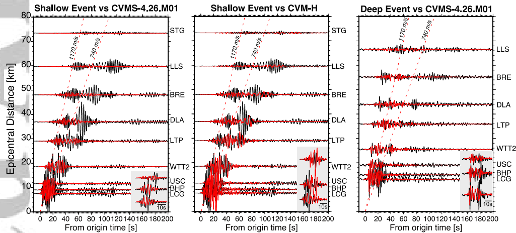
Figure 5. Record sections show the comparison between tangential velocity data (in black) for the Beverly Hills-Westwood pair and the 3D synthetics (in red) generated from model CVM-S.4.26.M01 (left and right column) and CVM-H (middle column). The waveforms are filtered at two different period ranges, 5 – 10 seconds (top row) and 2 – 10 seconds (bottom row). Each section is plotted on a common amplitude scale. The waveforms for the deep event (right column) are multiplied by a factor of 5 as the amplitude is weaker. For visual clarity, the waveforms in the gray box are scaled versions of waveforms at stations USC (top), BHP (middle) and LCG (bottom). The 3D synthetics are generated using an attenuation scaling of Q_s = 50V_s . Record section of CVM-H synthetics for the Westwood event is in the Supporting Information.
