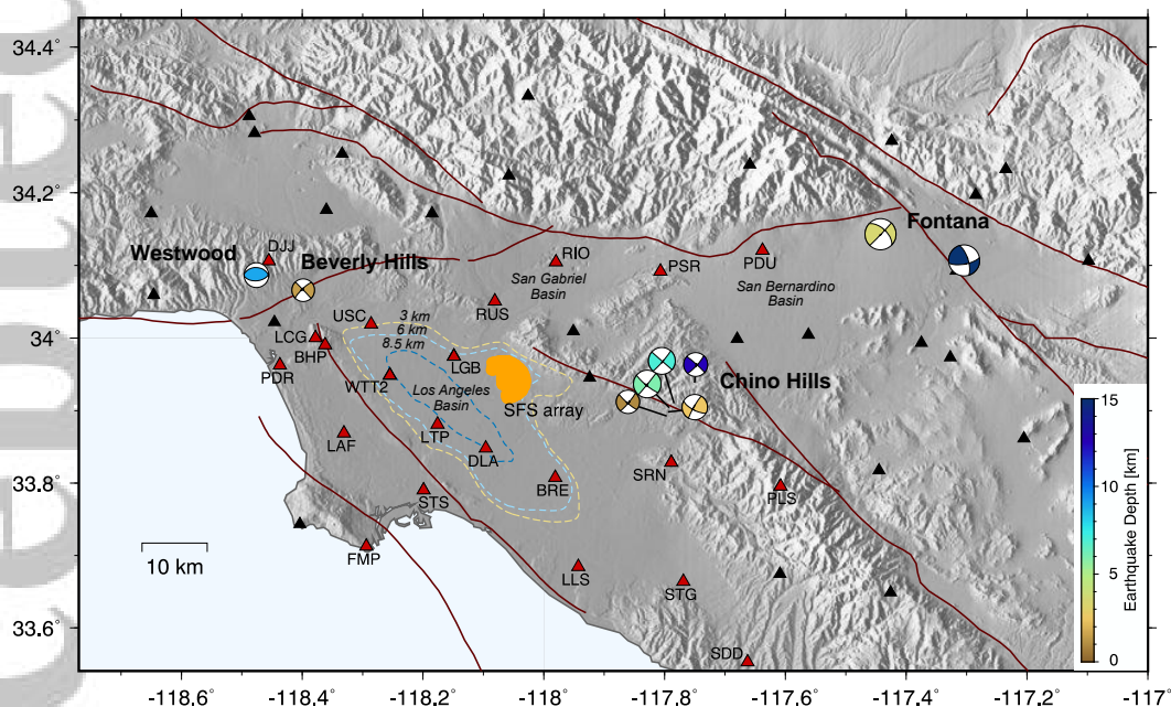
Figure 1. Map shows the location of earthquakes: the Beverly Hills-Westwood pair and Chino Hills series, directly sampling the Los Angeles basin, and the Fontana pair, sampling the San Bernardino, San Gabriel and Los Angeles basins. The earthquakes are color-coded by their depths. Triangles represent available broadband stations from the Southern California Seismic Network (SCSN; CI network code). Stations highlighted in this study are colored in red. The temporary Santa Fe Springs (SFS) dense array is in orange. The contour lines outline
