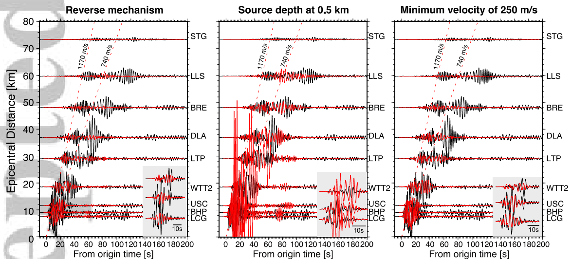
Figure 6. Record sections show the comparison between the tangential velocity data from the Beverly Hills event (black) and the 3D synthetics generated from CVM-S.4.26.M01 (red) using three different settings: choosing a reverse source mechanism instead of strike-slip (left), setting the source depth at 0.5 km instead of 1.5 km (middle), and using a velocity model with minimum velocity set at 250 m/s instead of 500 m/s. Waveforms are filtered at 5-10 seconds and 2 – 10 seconds and plotted in absolute amplitude. For visual clarity, the waveforms in the gray box are scaled versions of waveforms at stations USC (top), BHP
