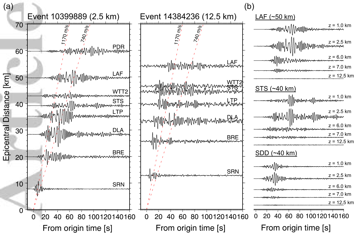
Figure 3. (a) Record sections show the tangential velocity data recorded by stations in the Los Angeles basin for the Chino Hills events 10399889 at 2.5 km depth (left) and 14384236 at 12.5 km (right). The waveforms are filtered at period 2 - 10 seconds and the amplitudes are scaled using station SRN. The dashed lines indicate wave packets traveling at 1170 m/s and 740 m/s, as shown in Figure 2. The record sections for all the events are in the Supporting Information. (b) Figure shows tangential velocity waveforms recorded at stations LAF, STS and SDD amplitudes for all the Chino Hill events. The waveforms are filtered at a period range of 2 - 10 seconds and the amplitudes are scaled by the amplitude at the deepest event (12.5 km). Stations LAF and STS are located near Los Angeles basin, and SDD is to the south, with a travel path completely outside the basin (see exact locations in Figure 1)
