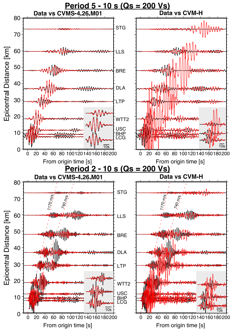
Figure 7. Record sections show the comparison between tangential velocity data (in black) for the Beverly Hills event and 3D synthetics (in red) generated from model CVM-S.4.26.M01 (left column) and CVM-H (right column). The waveforms are filtered at a period range 5 – 10 seconds (top row) and 2 – 10 seconds (bottom row). The 3D synthetics are generated using a weaker attenuation scaling of Q_s = 200V_s . For visual clarity, the waveforms in the gray box are scaled versions of waveforms at stations USC (top), BHP (middle) and LCG (bottom).
