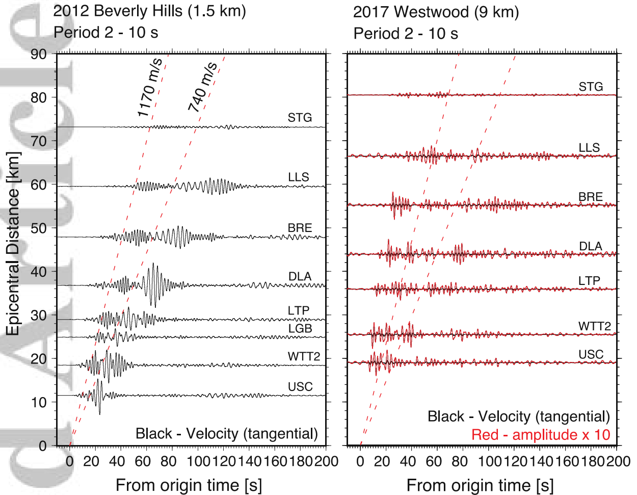
Figure 2. Record sections show the tangential velocity data recorded by stations across the Los Angeles basin for the Beverly Hills (left) and Westwood (right) events. The waveforms are filtered at a period range of 2 - 10 seconds and plotted on a common absolute scale. The waveform amplitudes for the Westwood event are significantly weaker, hence for better visuals, the waveforms are scaled by a factor of ten (shown in red). The dashed red lines indicate the arrivals of initial surface waves and later strong prolonged shaking, traveling at 1170 m/s and 740 m/s. Similar plots for radial and vertical velocities are in the Supporting Information.
