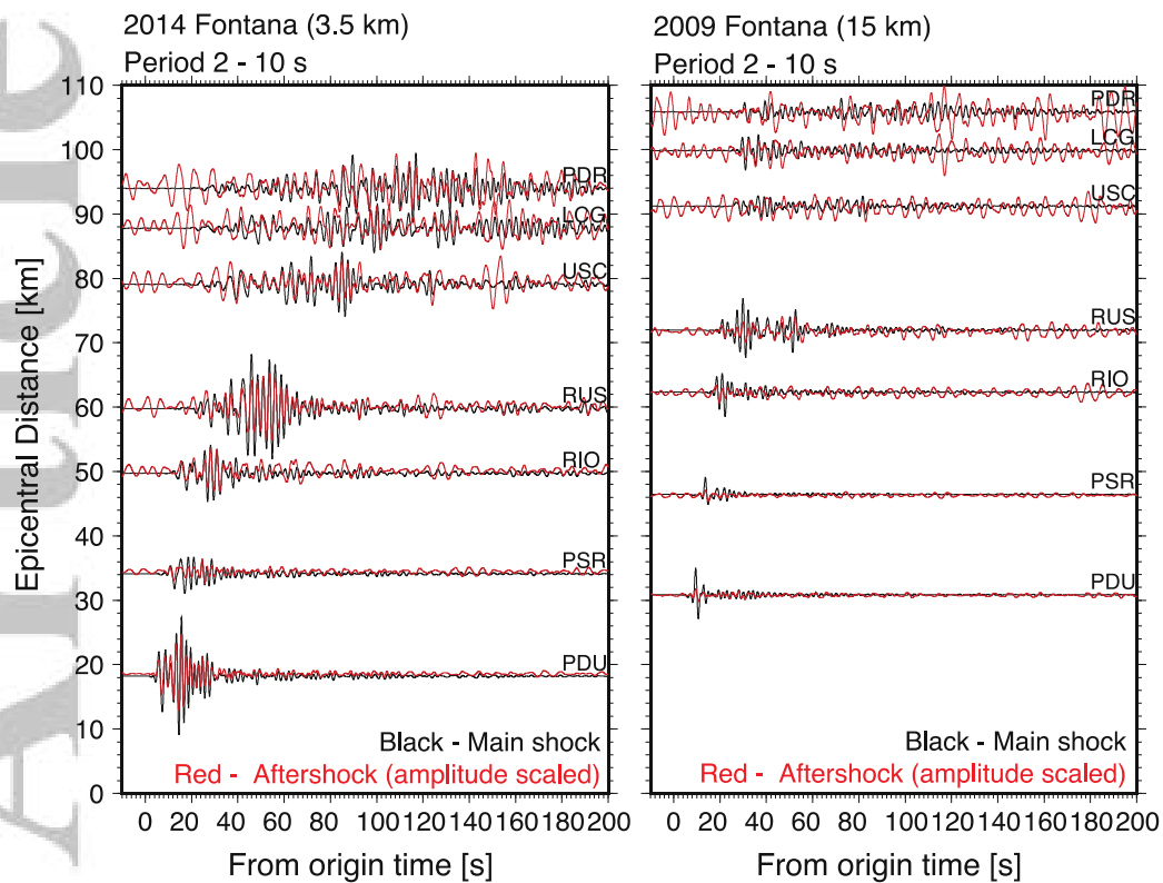
Figure 4. Record sections show the tangential velocity data for the Fontana pair (in black) and their respective M3 aftershocks (in red and scaled with a constant). The waveforms are filtered at a period range of 2 - 10 seconds. The station profile is approximately east to west, sampling the San Bernardino, San Gabriel and Los Angeles basins across the Whittier Narrows (near RUS).
