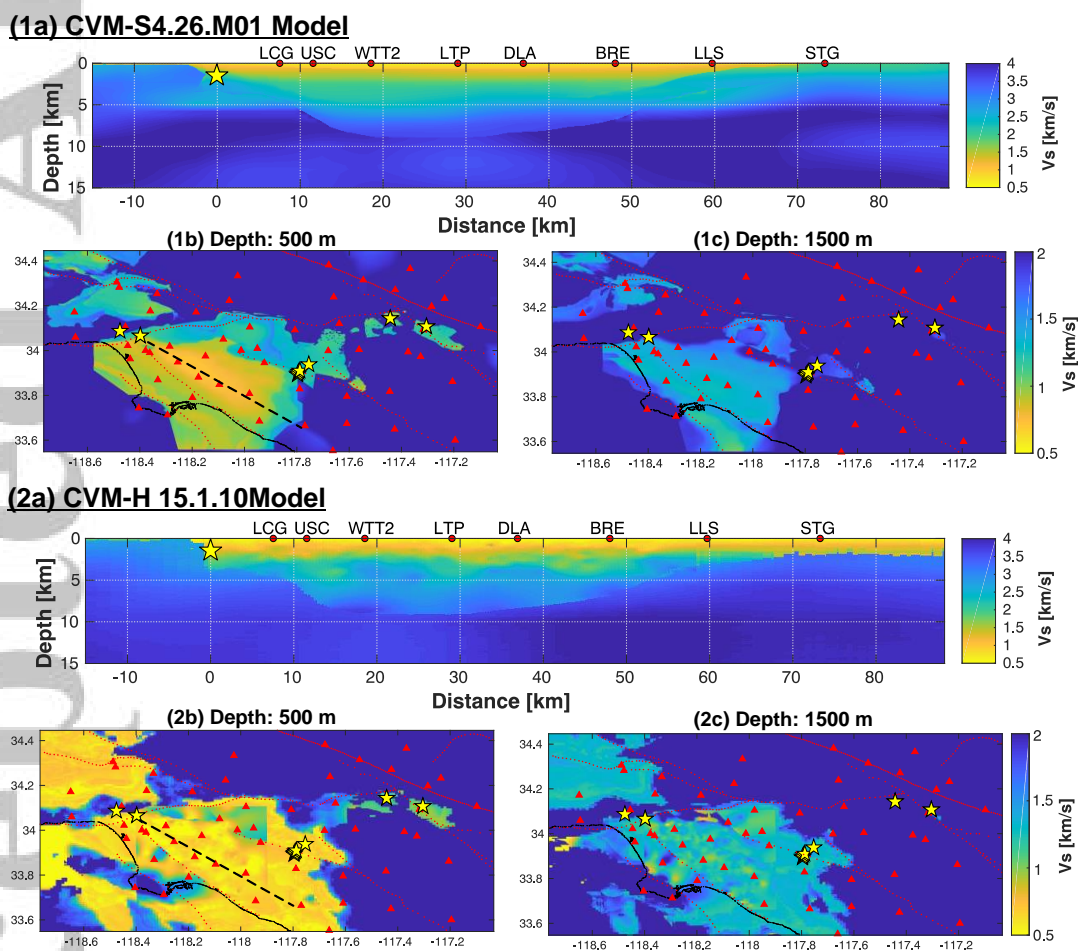
Figure 8. (top panel, 1a) Cross-section showing the shear wave velocity structure from the CVM-S4.26.M01 model across the Los Angeles Basin, stations (red) along the profile and the depth of the 2012 Beverly Hills shallow event (yellow star). Maps show horizontal depth profile of the CVM-S4.26.M01 model at depth 500 m (1b) and 1500 m (1c). The black dashed line shows the location of the cross-section profile. Locations of earthquakes (yellow stars) and seismometers (red triangles) are shown as well. Red lines delineate the known
