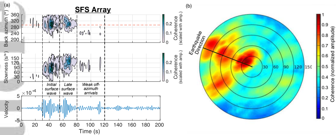
Figure 9. (a) The back azimuth and slowness of P-, S- and surface wave arrivals from the Beverly Hills event at the Santa Fe Springs (SFS) array located 35.5 km away from the epicenter. The coherence is scaled with amplitude to highlight stronger shaking. The earthquake is at a back-azimuth of 291 degrees. The vertical-component velocity seismogram recorded by one of the stations in the center of the SFS array is also shown. The seismogram is bandpass filtered between 2 – 10 seconds with a two-pass Butterworth filter. (b) Polar plots showing the data coherence, stacked over the entire 200-second duration. The amplitude is normalized in order to show the weak yet coherent arrivals. Warmer color indicates higher coherence. Most coherent energy is confined to the great circle path. There is some coherent energy observed arriving from off-great circle azimuths at times of 80 to 120 seconds.
