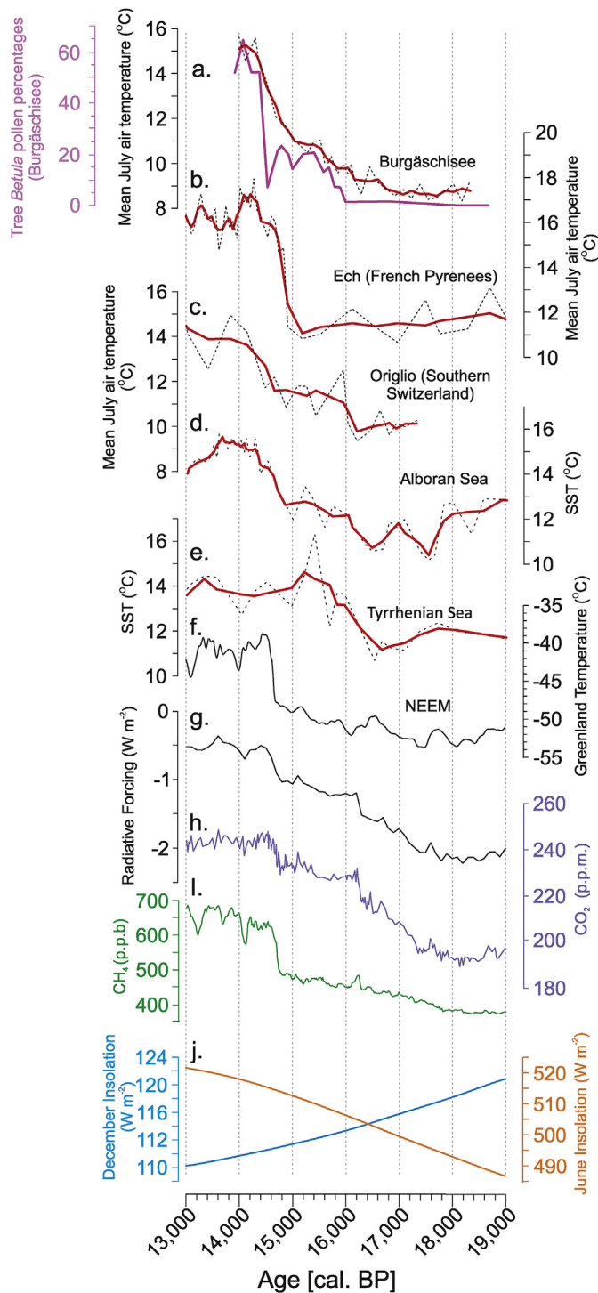
Fig. 6. Palaeotemperature records for the early Late Glacial. For temperature records (plots a. - e.) the dashed black line represents unsmoothed values whereas the solid red line represents a three sample running average. a. Burgäschisee chironomid temperature record from the Swiss lowlands and Burgäschisee tree Betula pollen percentages (solid pink line, Rey et al., 2017); b. Ech Palaeolake chironomid-inferred temperature (Data digitized from Millet et al., 2012); c. Lago di Origlio chironomid-inferred temperature (Samartin et al., 2012); d. Alboran sea surface temperature (SST; Cacho et al., 2001); e. Tyrrhenian SST (Cacho et al., 2001); f. NEEM temperature reconstruction (Buizert et al., 2014); g. Total radiative forcing from greenhouse gasses (Schilt et al., 2010; Marcott et al., 2014); h. CO 2 from West Antarctic Ice Sheet Divide ice core (WDC; Marcott et al., 2014); i. CH 4 from WDC (WAIS Divide Project Members, 2013; Marcott et al., 2014) and j. Summer and December insolation curves for 45°N (Berger and Loutre, 1991). (For interpretation of the references to colour in this figure legend, the reader is referred to the Web version of this article.)
