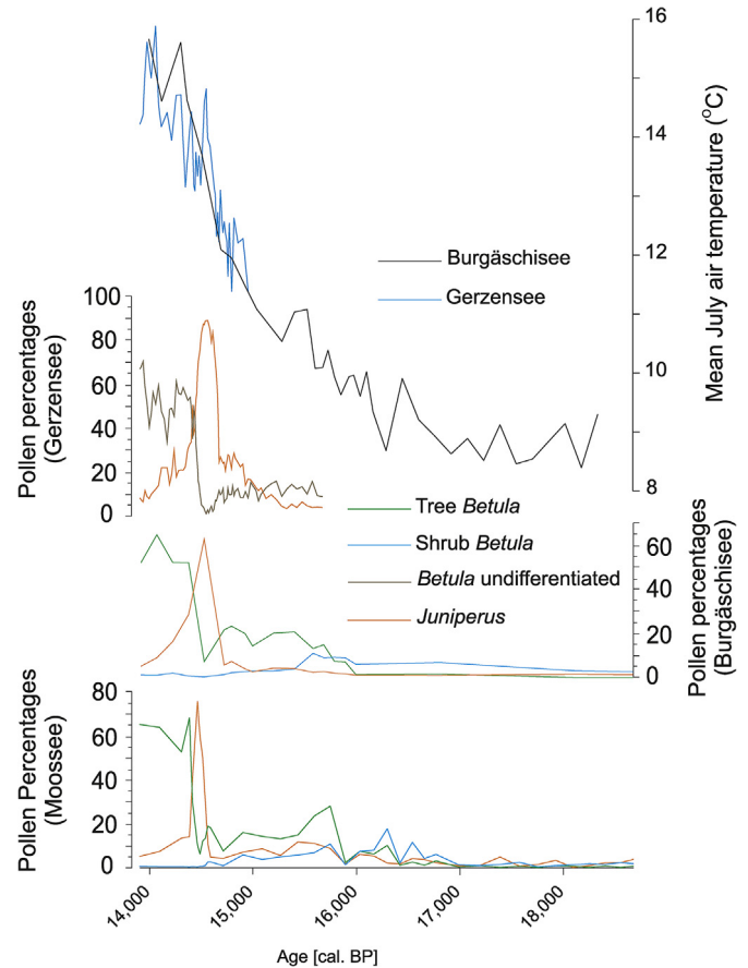
Fig. 5. Chironomid temperature reconstructions from the Northern Swiss Plateau corrected to 465 m a.s.l. (Burgäschisee, this publication; Gerzensee, Lotter et al., 2012) compared with selected pollen types in the Burgäschisee (Rey et al., 2017), Gerzensee (Ammann et al., 2013; shrub Betula nana was not separated from tree Betula pollen in this study) and Moossee (Rey et al., 2020) records. The Gerzensee record is presented on the age scale of van Raden et al. (2013). For the oldest section we only present samples within 300 years of the Oldest Dryas - Bölling transition, however, since this represents the lowest distinctive age tie point in the Gerzensee record, and lower sections are only very poorly constrained by the available chronological information.
